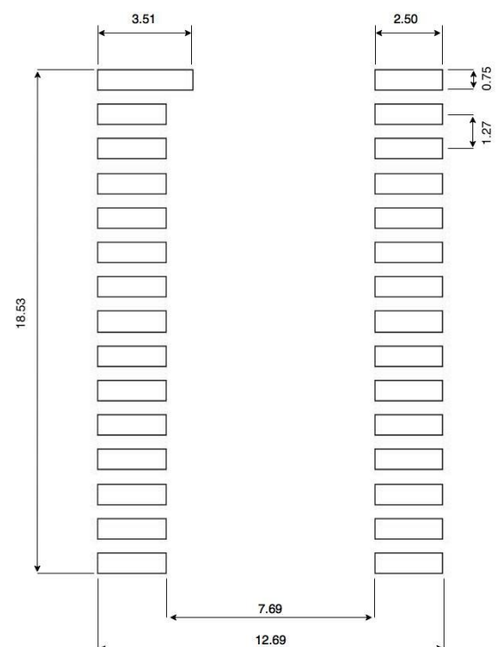
Figure 16: Recommended Pad Layout in mm (top view)
