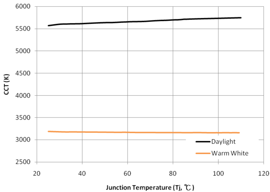
Fig.13 CCT vs junction temperature - White
