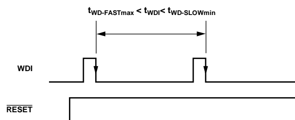
Figure 23. Normal Watchdog Operation
