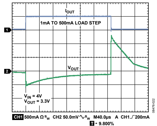
Figure 24. Load Transient Response, C_{OUT} = 1\text{ μF}
