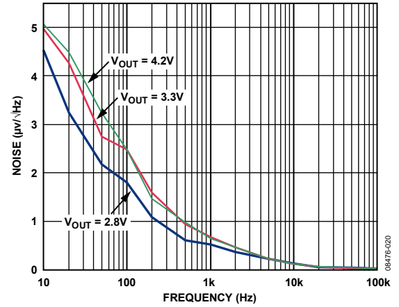
Figure 22. Output Noise Spectrum, V_{IN} = 5\text{ V}
