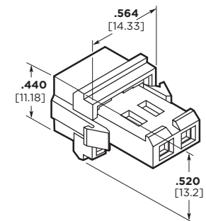
Two-Position Only 641533-1
