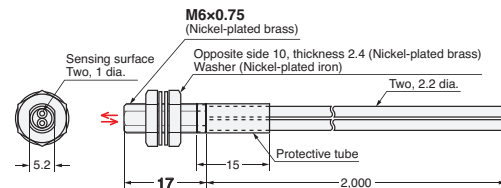
37-I E32-D11U 2M (Free Cutting)
