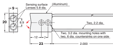
53-E E32-A09 2M (Free Cutting)
