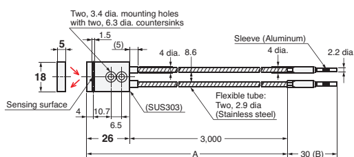
45-D E32-A08H2 3M (No Cutting)
