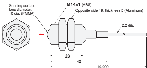
23-B E32-T14 2M (Free Cutting)
