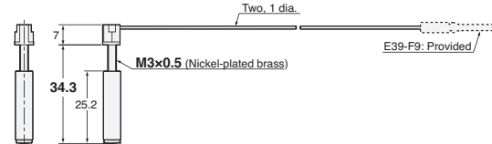
21-F E32-C31N 2M (Free Cutting) + E39-F3B
