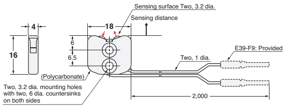
31-C E32-L25L 2M (Free Cutting)
