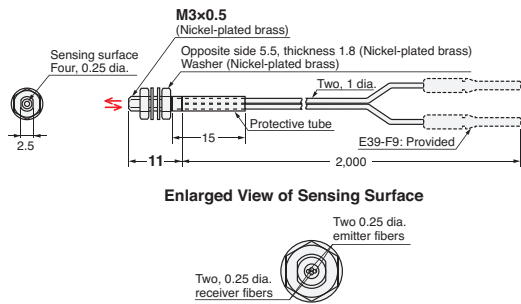
41-B E32-D21 2M (Free Cutting)
