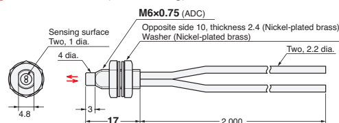
09-G E32-D11R 2M (Free Cutting)
