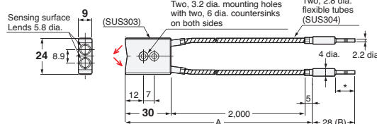
53-F E32-A09H2 2M (No Cutting)
