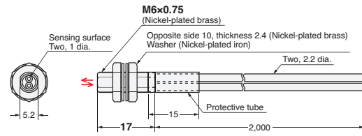
41-E E32-D11 2M (Free Cutting)
