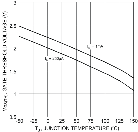
Figure 7 Gate Threshold Variation vs. Temperature
