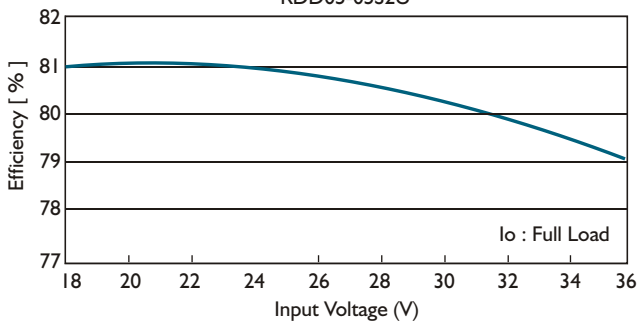
Efficiency Vs Input Voltage RDD05-05S2U
