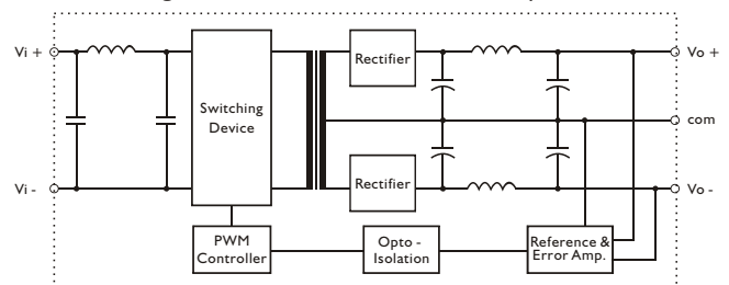
• Block diagram for RDD05U series with dual output
