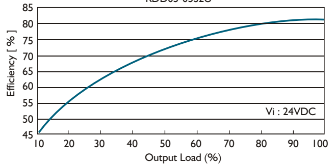
Efficiency Vs Output Load RDD05-05S2U
