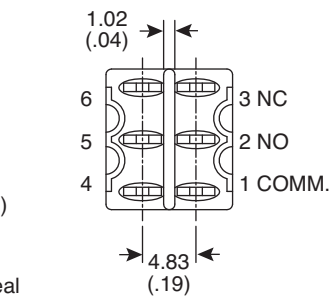
SWITCH FUNCTION
