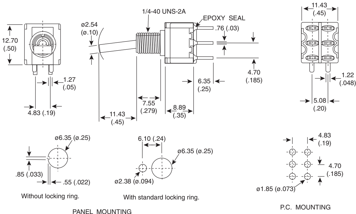
PANEL MOUNTING
