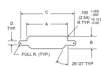
Figure 2 Rear Mounting
