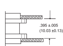
Plug and Receptacle Front Mounted
