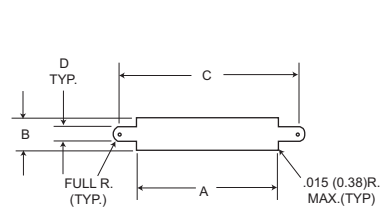
Figure 1 Front Mounting
