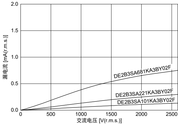
RA型 (AC500V (r.m.s.)) (B特性)
