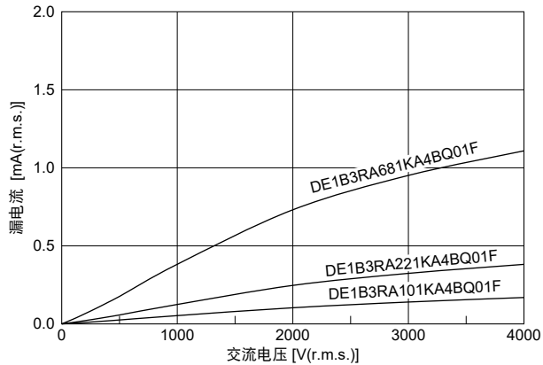
RA型 (AC500V (r.m.s.)) (B特性)
