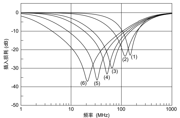
RA型 (AC250V (r.m.s.))
