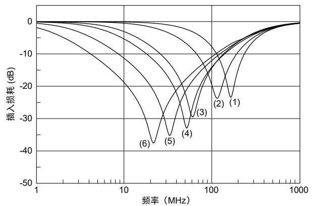
RA型 (AC500V (r.m.s.))
