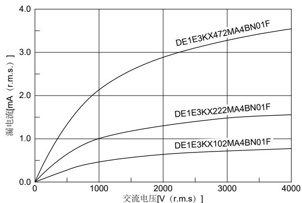
SA型 (AC250V (r.m.s.)) (E特性)
