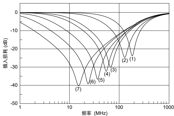
SA型 (AC250V(r.m.s.))
