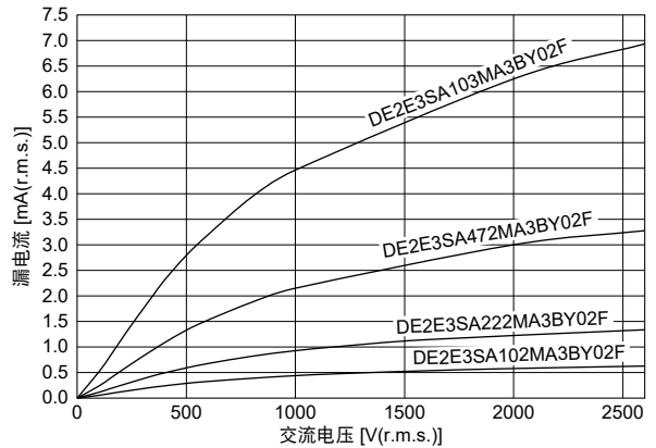
RA型 (AC500V (r.m.s.)) (E特性)
