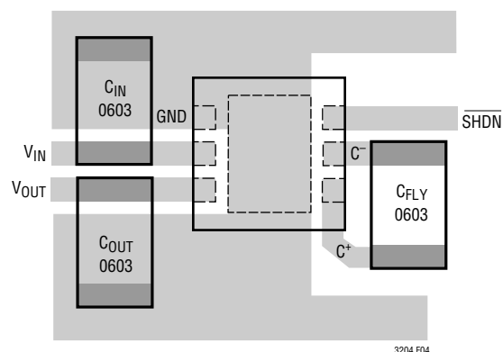
Figure 4. Recommended Layout
