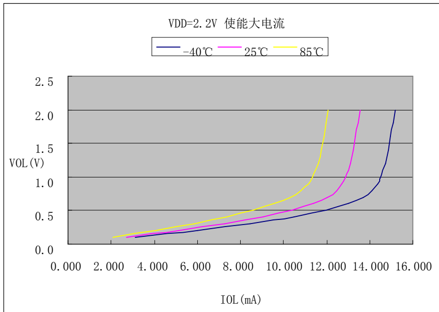
B: V_{OL} vs I_{OL} @VDD=2.2V
