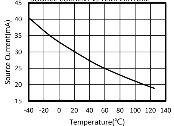
SOURCE CURRENT vs TEMPERATURE
