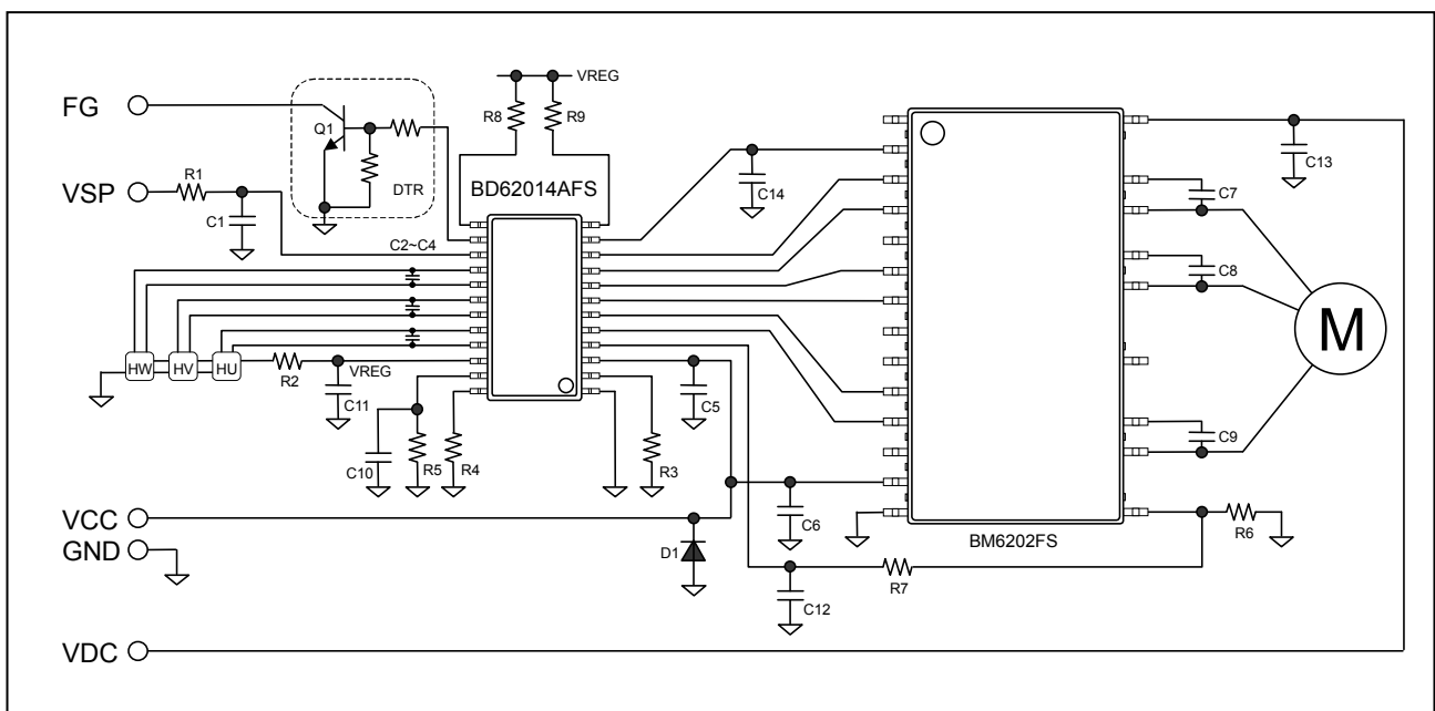
Figure 1. Application circuit example - BD62014AFS & BM6202FS
