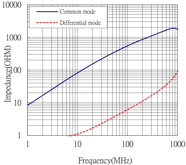
CMF2012F-601-2P-T
