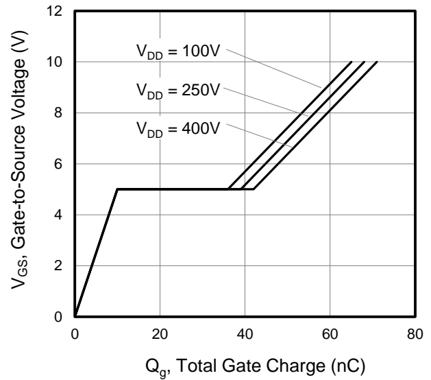
Figure 8. Gate Charge
