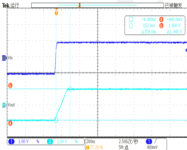
Slew Rate V DD =5V, G=1 (buffer), V IN =0~1V@1kHz Rise
