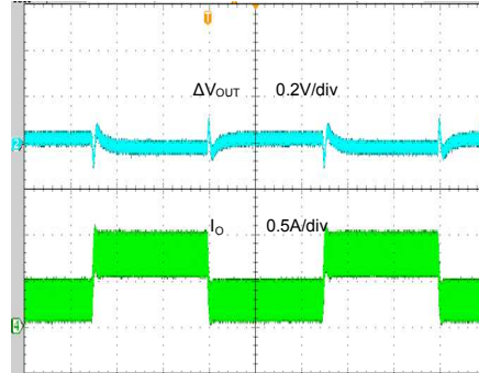
Time (400μs/div)
