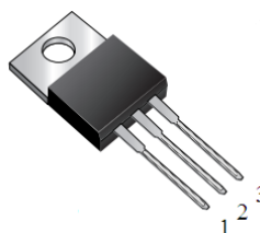
TO-220AB PS20U45S
