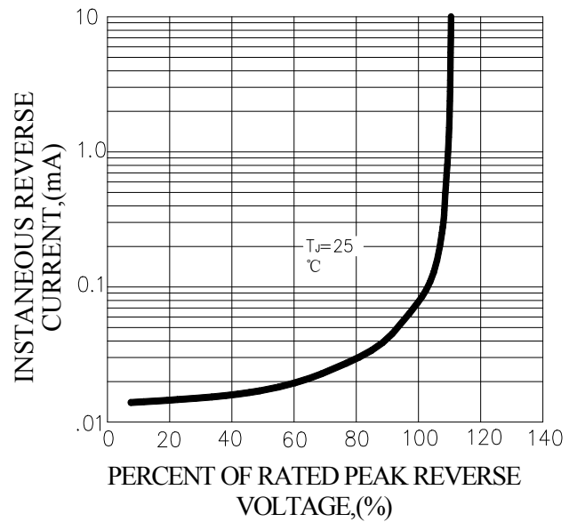
FIG.4-TYPICAL REVERSE CHARACTERISTICS
