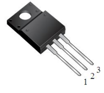
ITO-220AB PS30U100FCT
