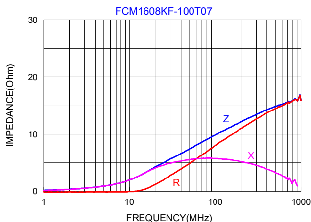
■ Impedance-Frequency Characteristics
