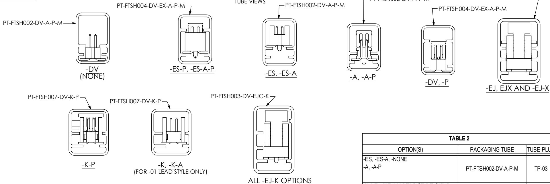
FIG 13 TUBE VIEWS
