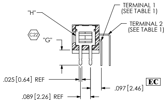
SECTION "J"-"J"
