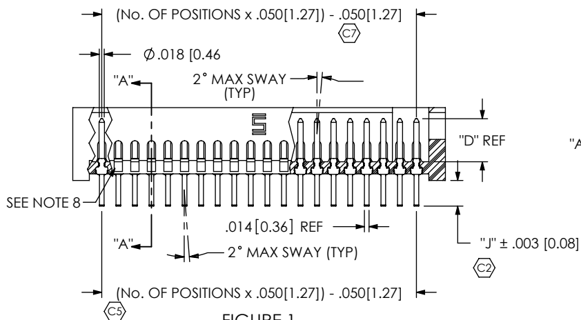
FIGURE 1 THROUGH HOLE -01, -03, -11, -13, -21, -23, -31
