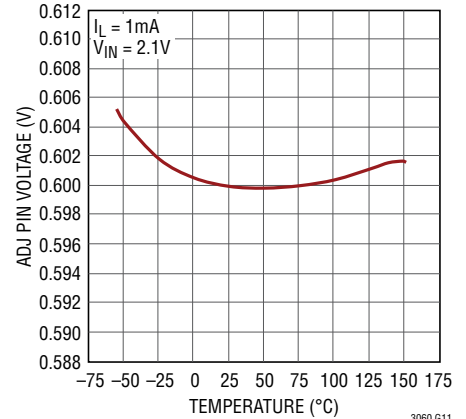
LT3060 ADJ Pin Voltage
