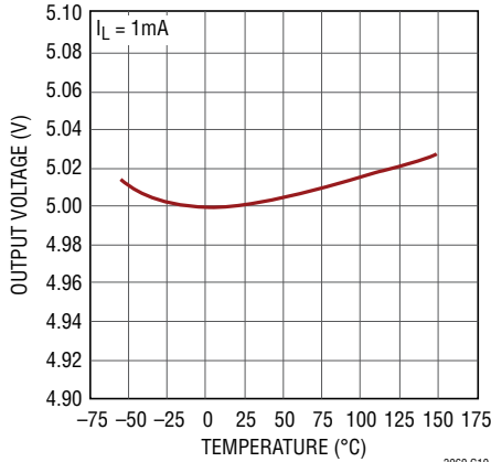
LT3060-5 Output Voltage
