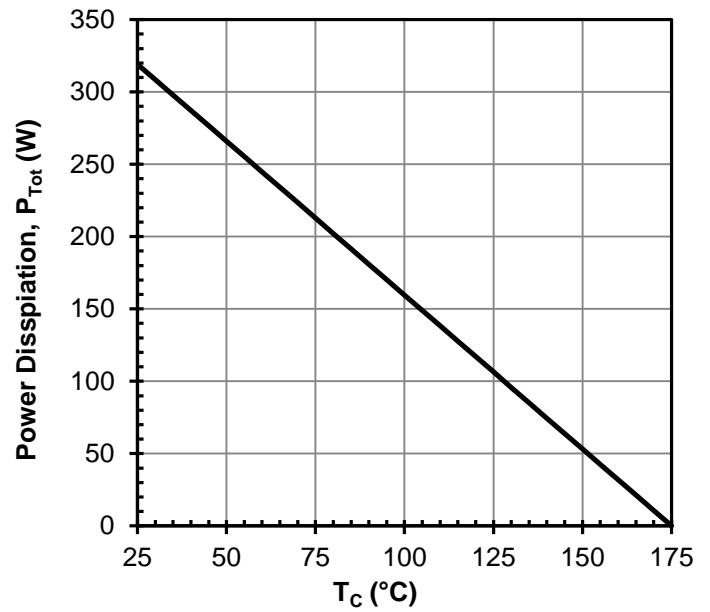
Figure 4 Power dissipation
