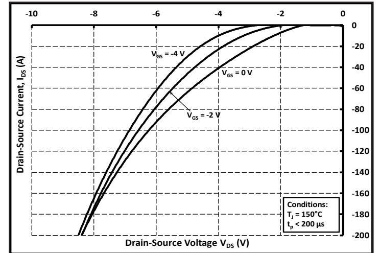
Figure 10. Body Diode Characteristic at 150^\circ\text{C}
