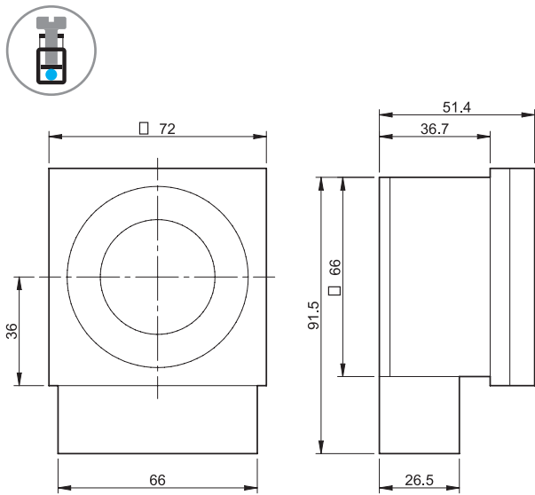
12.71 Screw terminal
