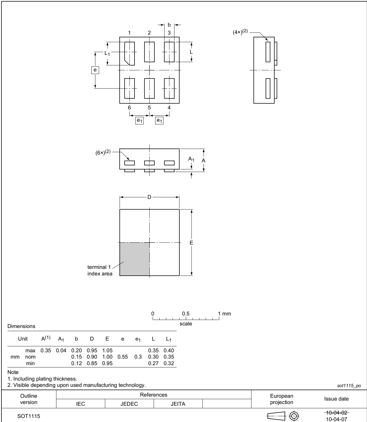
Fig 18. Package outline SOT1115 (XSON6)
