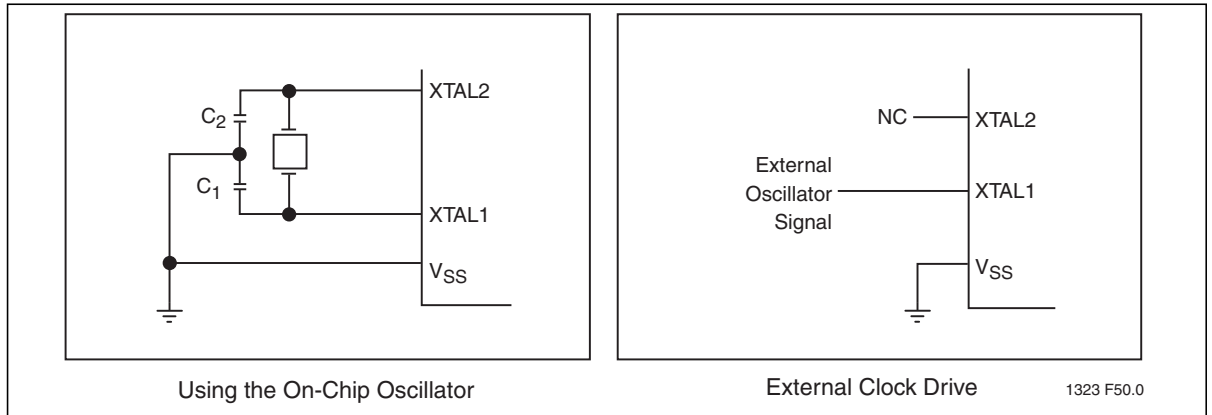
Figure 26: Oscillator Characteristics
