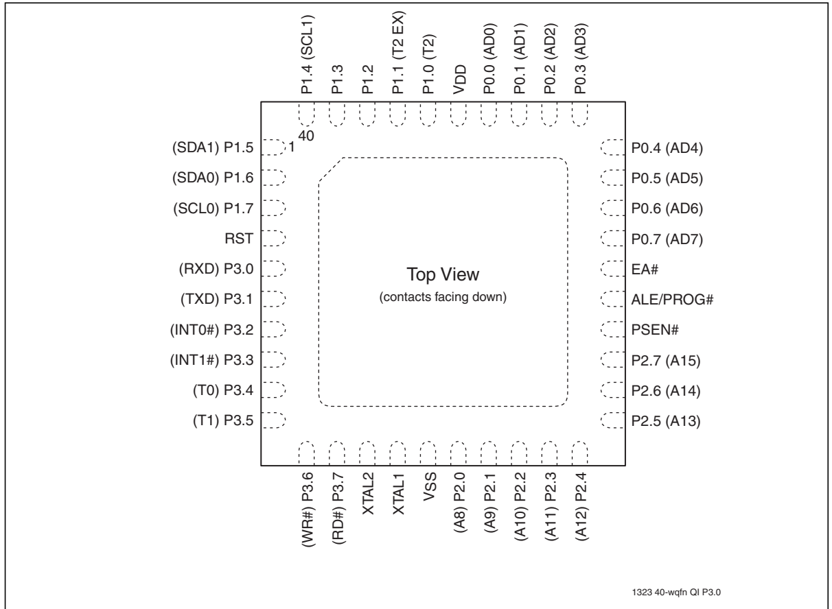
Figure 4: Pin Assignments for 40-Contact WQFN
