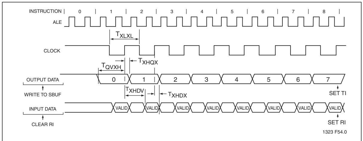
Figure 30: Shift Register Mode Timing Waveforms
