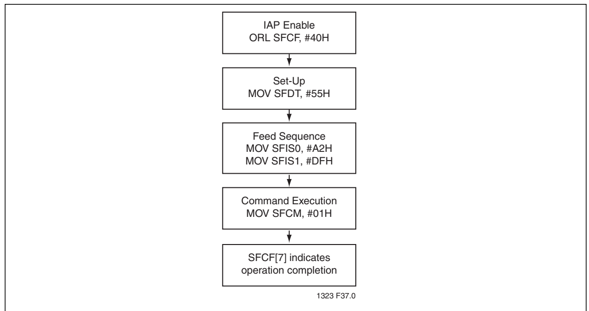
Figure 8: Chip-Erase
