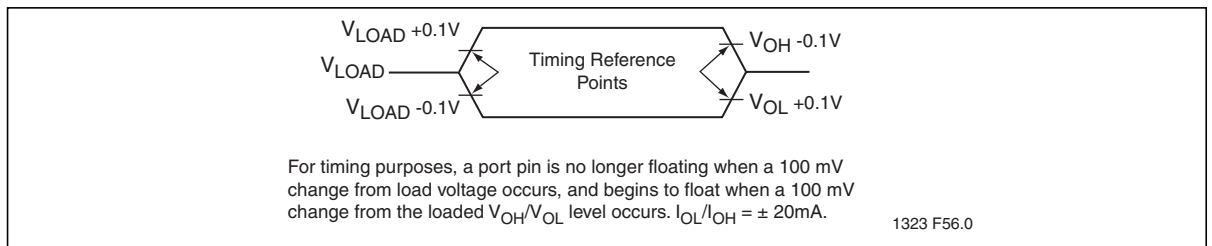
Figure 32: Float Waveform
