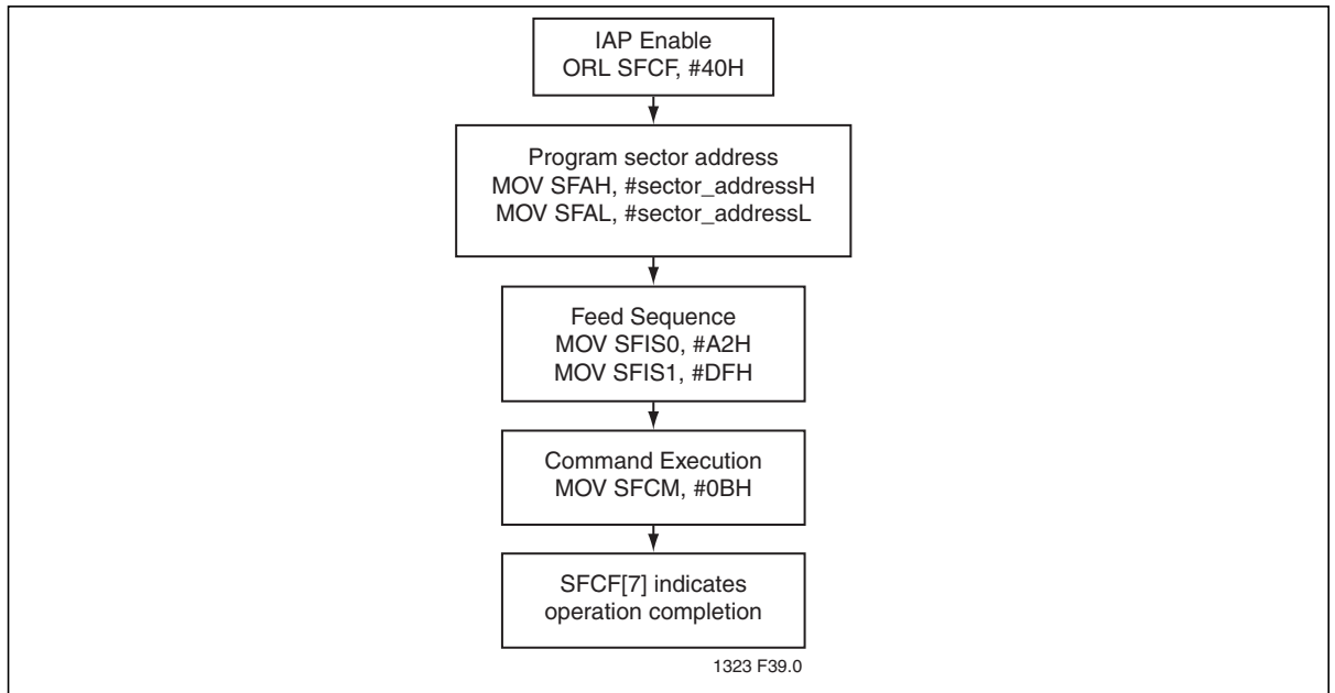
Figure 10: Sector-Erase
