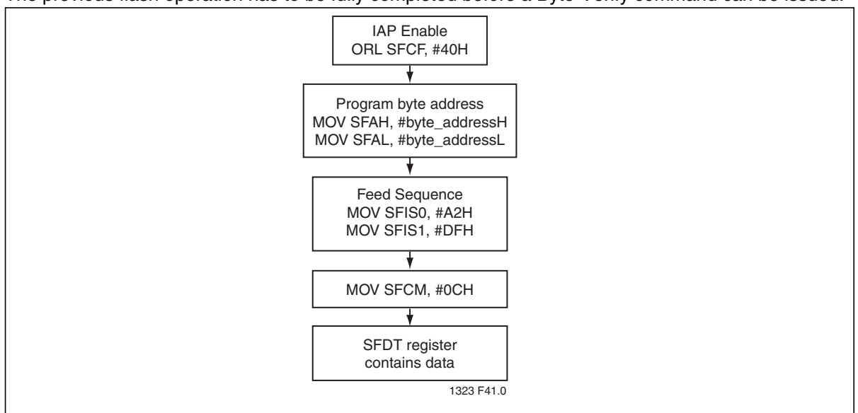
Figure 12: Byte-Verify
