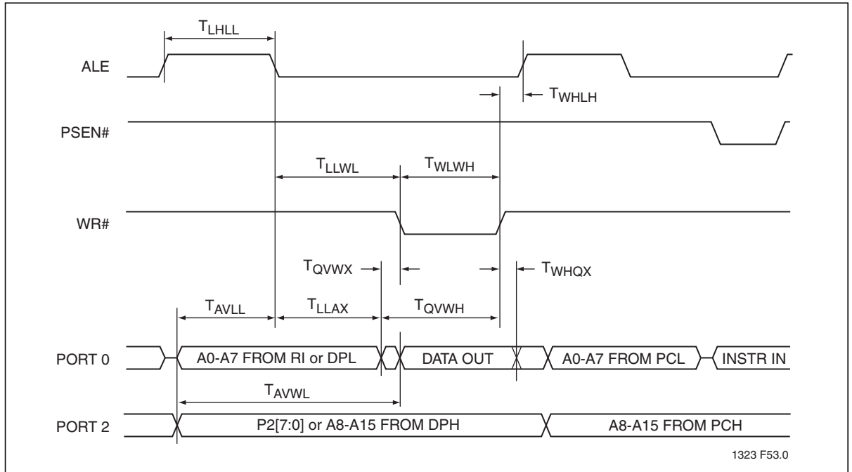
Figure 29: External Data Memory Write Cycle
