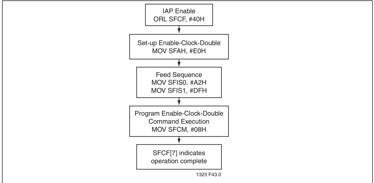
Figure 14: Enable-Clock-Double
