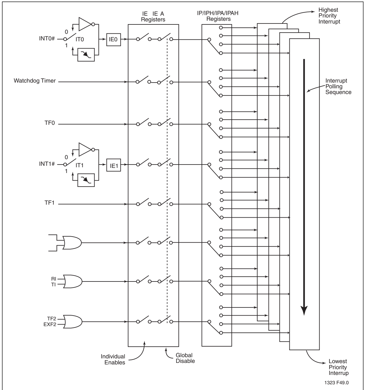
Figure 25: Interrupt Sequence
