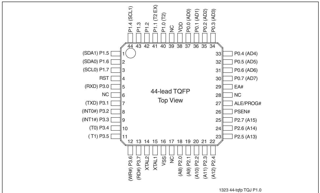
Figure 2: Pin Assignments for 44-Lead TQFP
