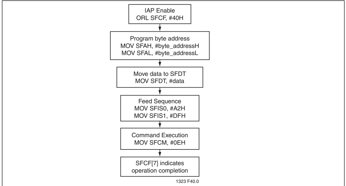
Figure 11: Byte-Program
