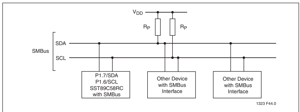
Figure 20: Typical SMBus Configuration
