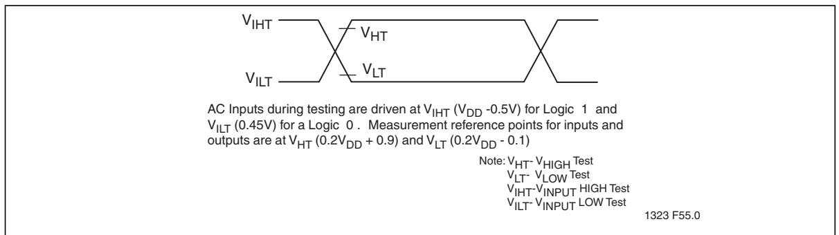
Figure 31: AC Testing Input/Output Test Waveform
