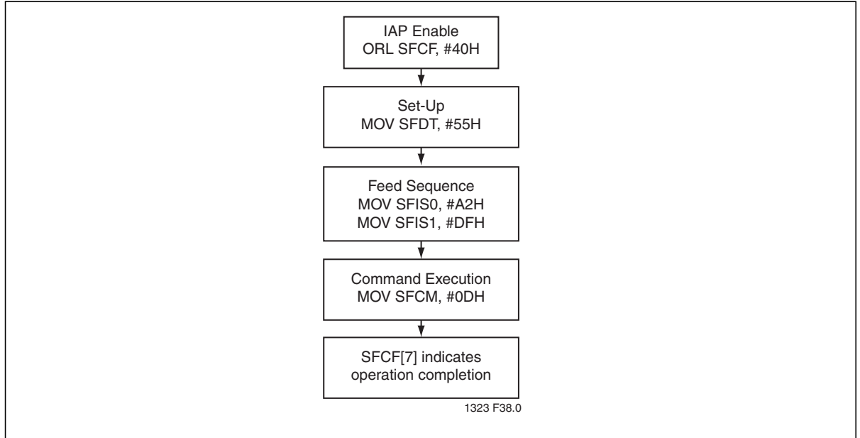
Figure 9: Partition0-Erase
