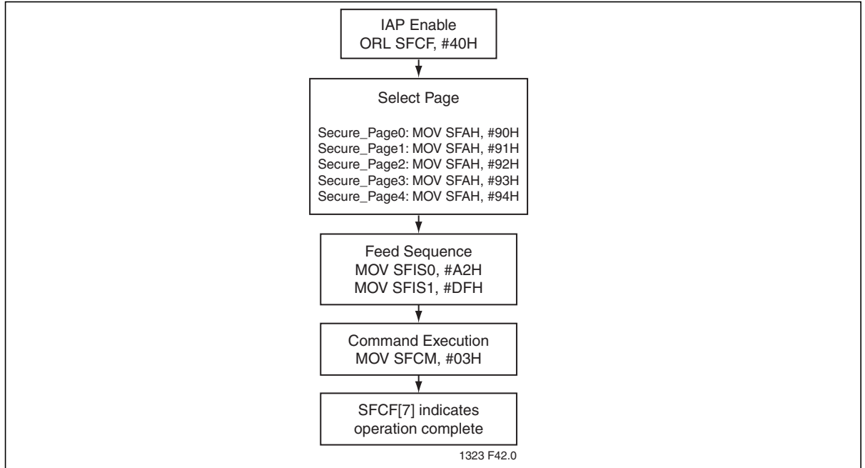
Figure 13: Secure-Page0-4
