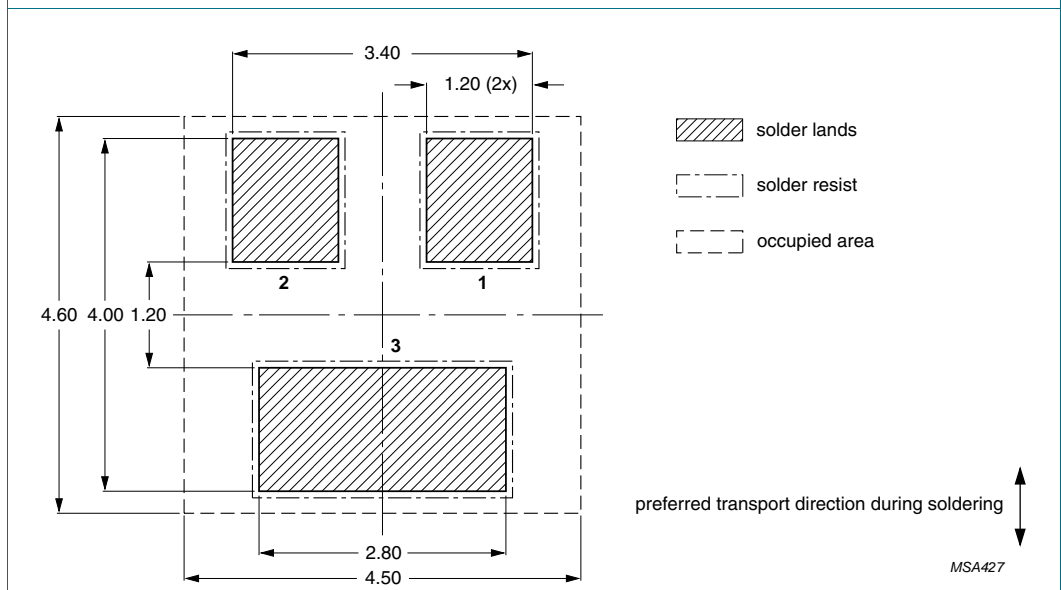
Fig 7. Reflow soldering footprint SOT23 (TO-236AB)
