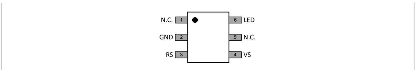
Figure 2 Pinout BCR430
