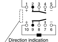
2-coil latching
