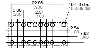
PC board pattern (Copper-side view)
