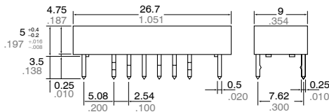
Self-clinching terminal
