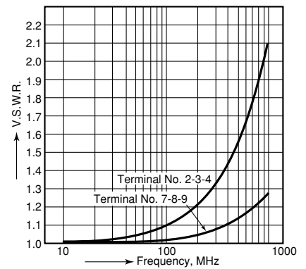
15-(3). High-frequency characteristics
