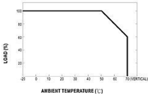
■ Derating Curve
