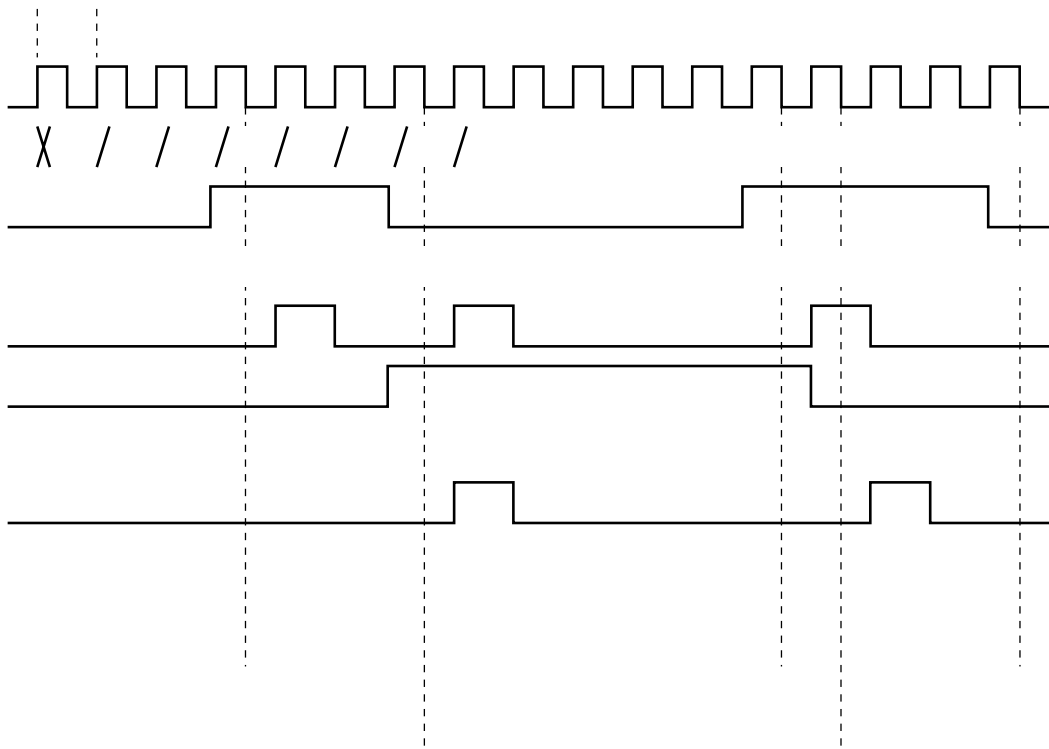
Figure 6-22. Timing of Pulse Width Measurement Operation with Free-Running Counter (with Both Edges Specified)
