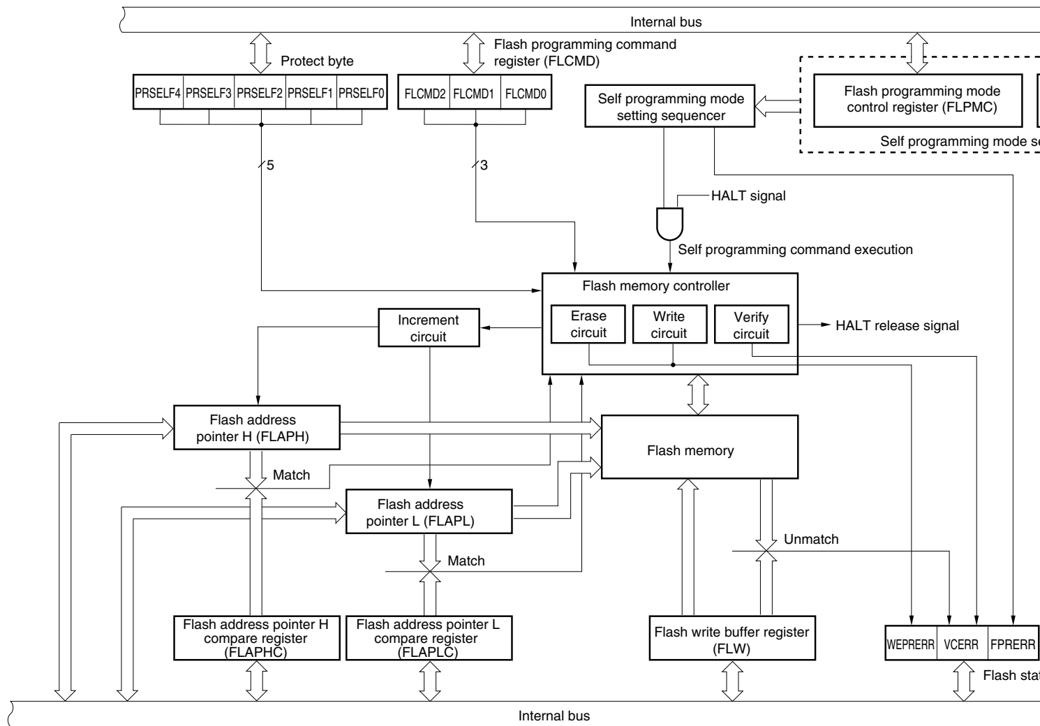
Figure 18-8. Block Diagram of Self Programming
