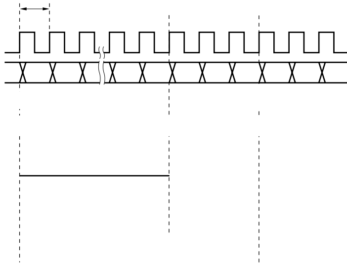
Figure 6-31. PPG Output Operation Timing
