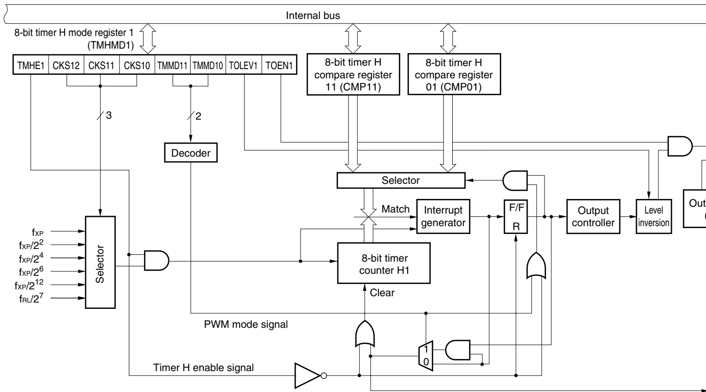
Figure 8-1. Block Diagram of 8-bit Timer H1
