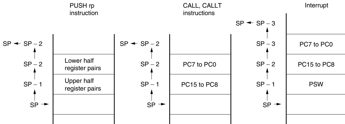
Figure 3-8. Data to Be Saved to Stack Memory
