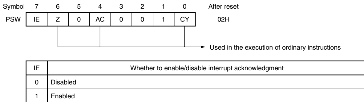
Figure 12-6. Program Status Word (PSW) Configuration
