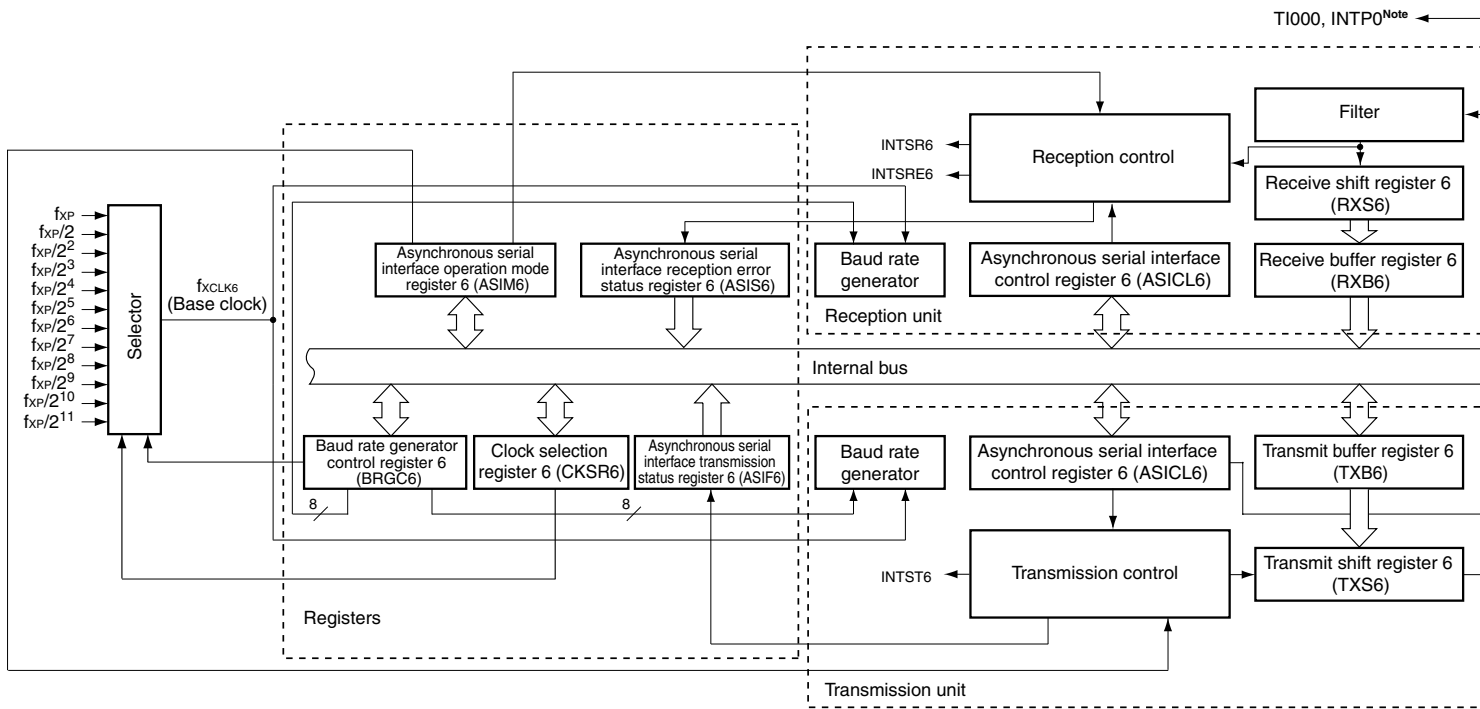
Figure 11-4. Block Diagram of Serial Interface UART6
