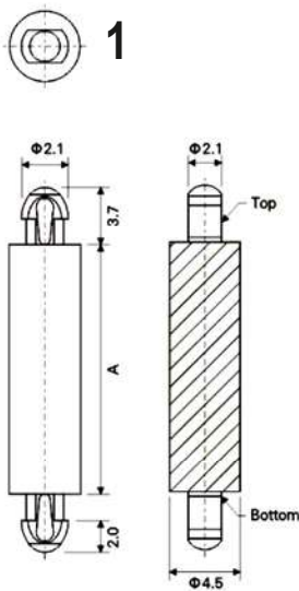
Top & Bottom Hole \varnothing 2.5 \pm 0.05 mm Top & Bottom Panel Thickness 1.57 mm Type 1
