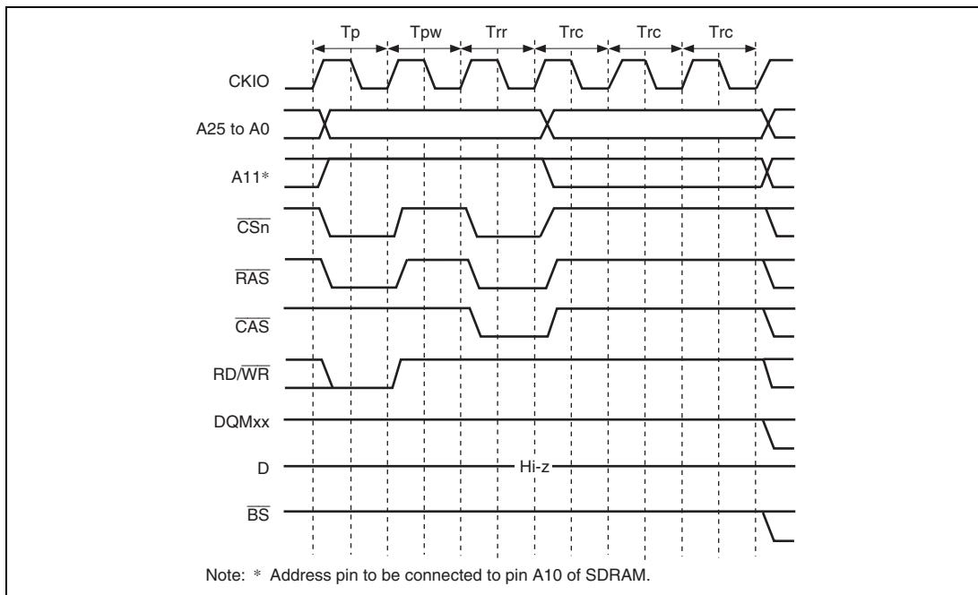
Figure 7.25 Auto-Refreshing Timing
