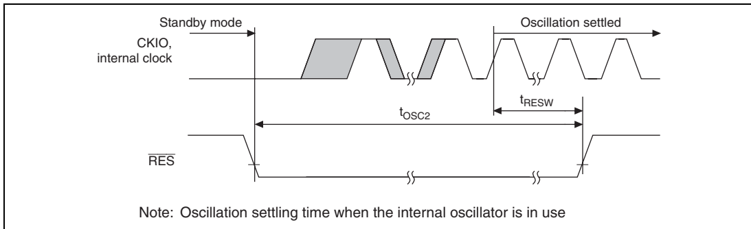
Figure 25.4 Oscillation Settling Timing after Standby Mode (By Reset)
