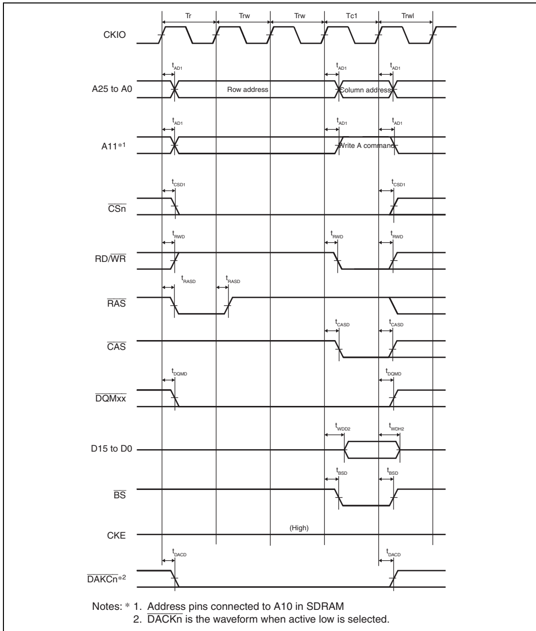
Figure 25.21 Synchronous DRAM Single Write Bus Cycle (Auto-Precharge, WTRCD = 2 Cycles, TRWL = 1 Cycle)
