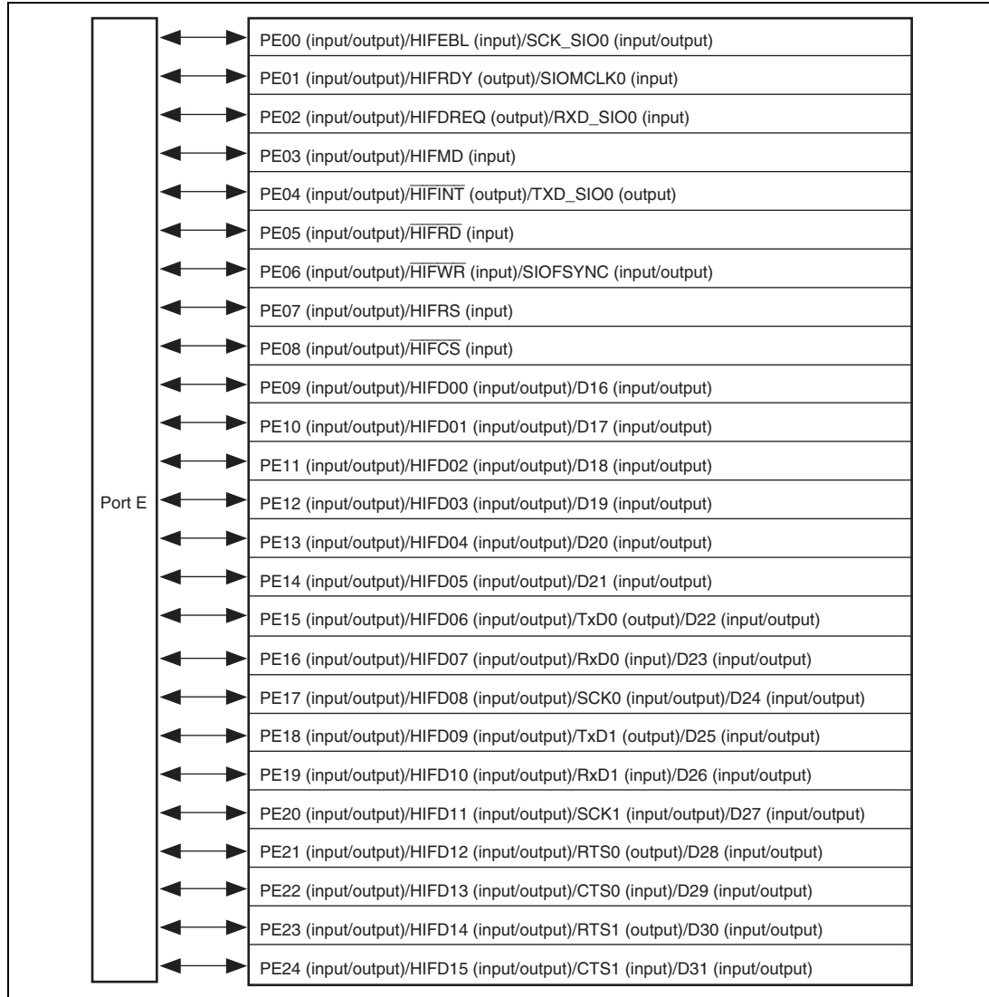
Figure 19.5 Port E
