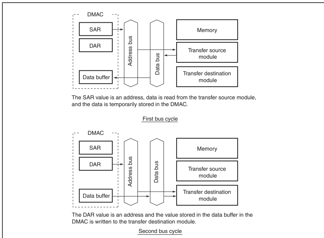
Figure 13.5 Data Flow of Dual Address Mode
