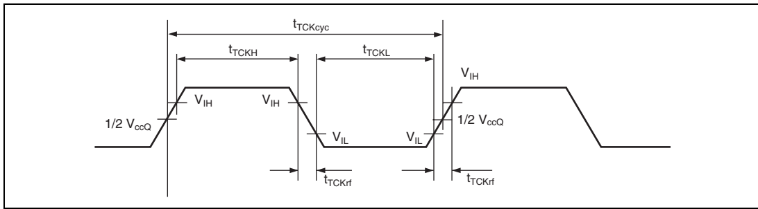
Figure 25.59 TCK Input Timing
