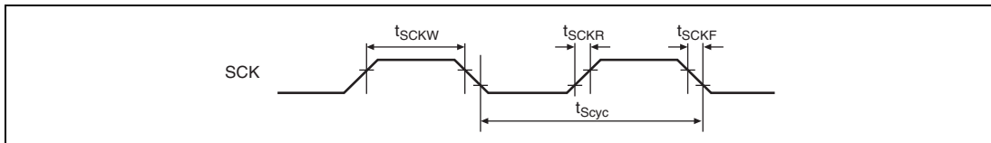
Figure 25.39 SCK Input Clock Timing
