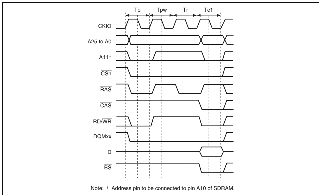
Figure 7.24 Single Write Timing (Bank Active, Different Row Addresses)
