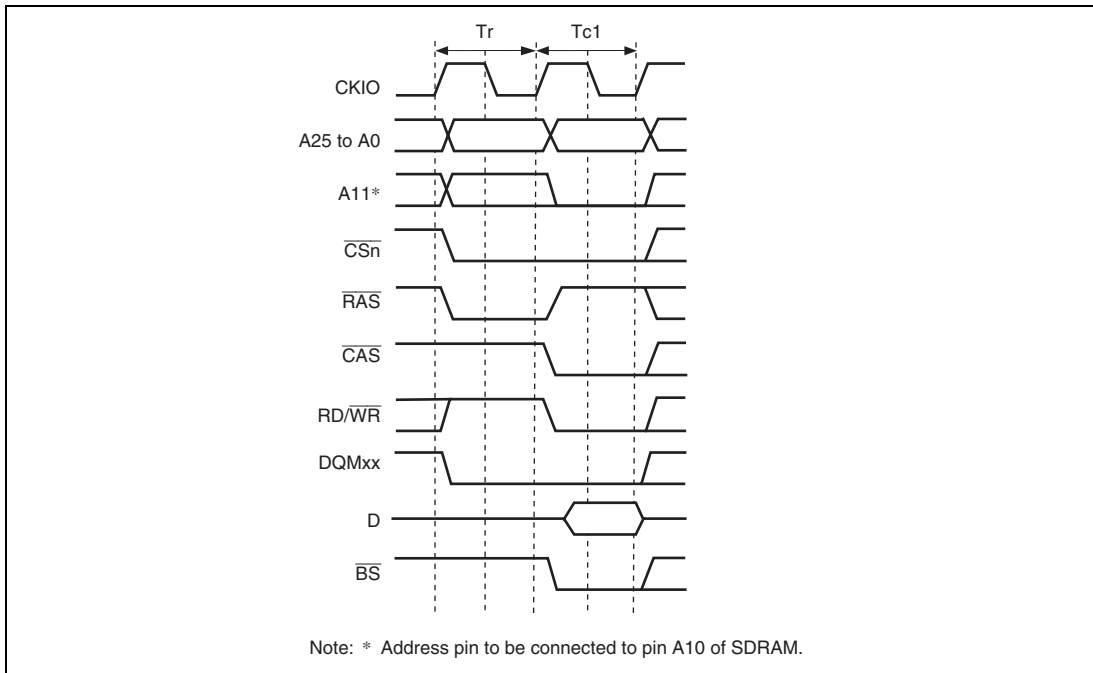
Figure 7.22 Single Write Timing (No Auto Precharge)
