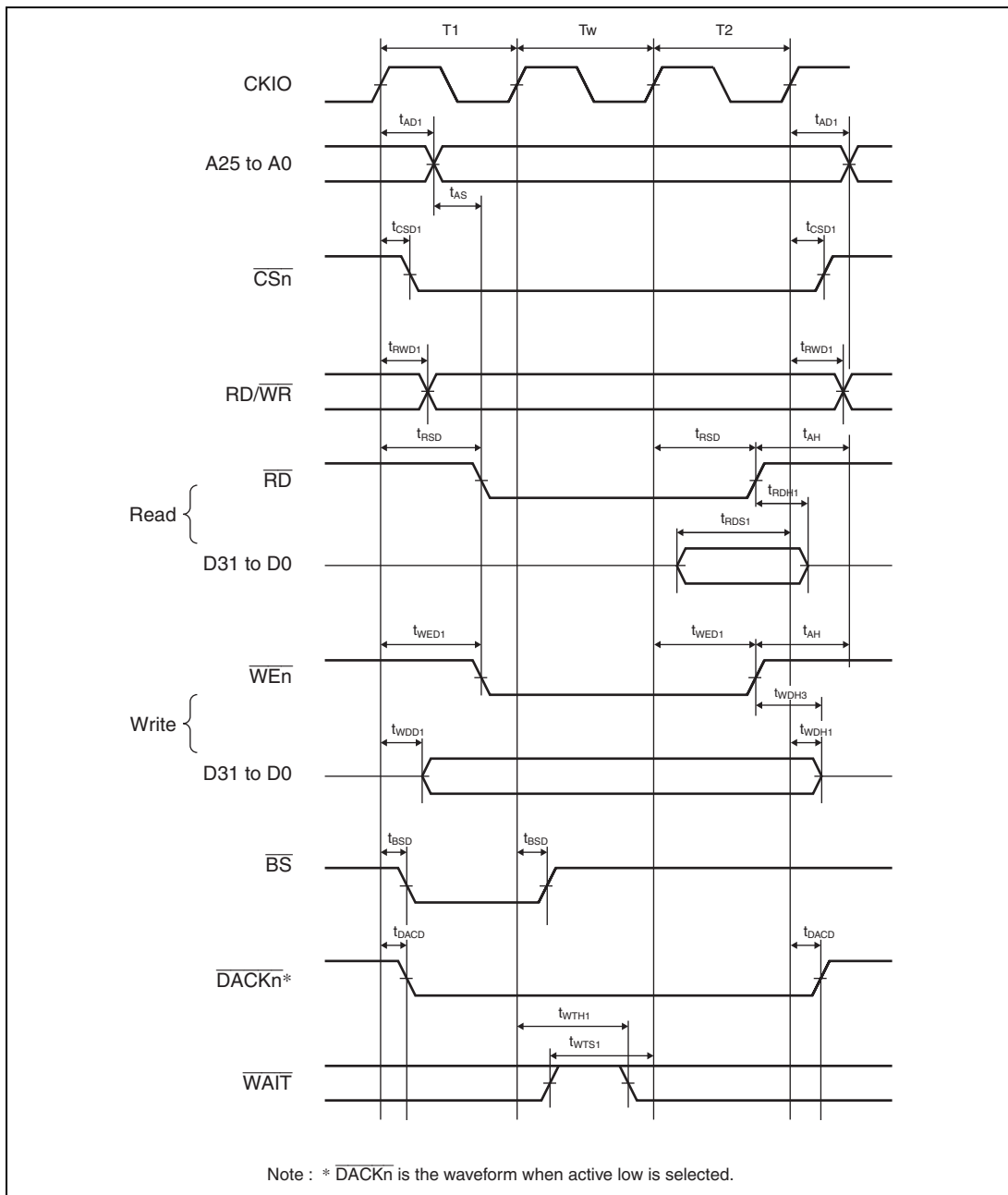
Figure 25.11 Basic Bus Timing: One Software Wait Cycle
