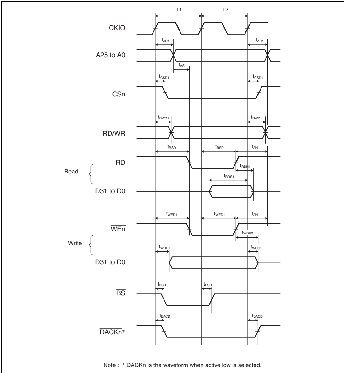
Figure 25.10 Basic Bus Timing: No Wait Cycle
