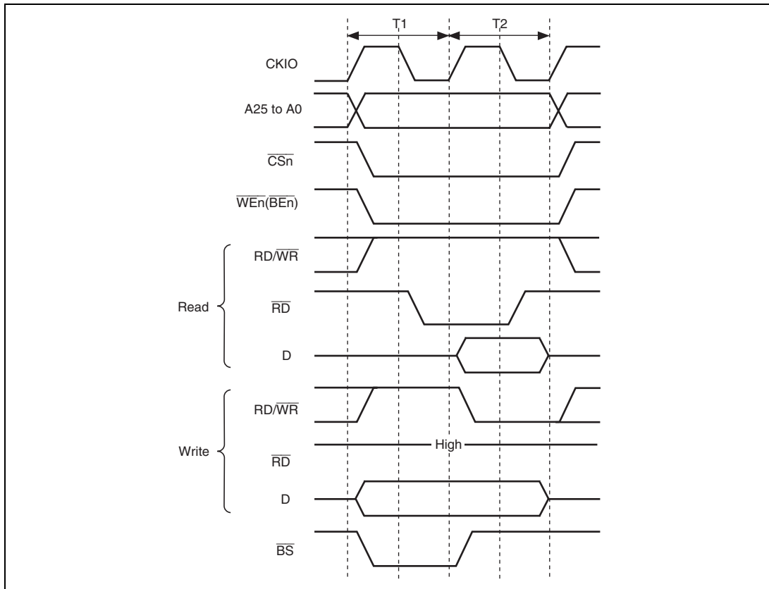
Figure 7.29 Basic Access Timing for Byte-Selection SRAM (BAS = 1)
