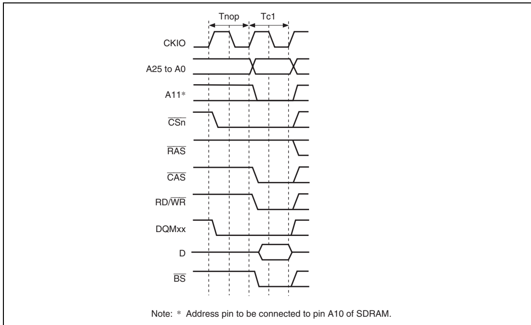
Figure 7.23 Single Write Timing (Bank Active, Same Row Address)
