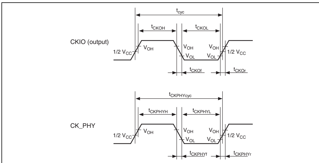
Figure 25.2 CKIO Clock Output Timing and CK_PHY Clock Input Timing
