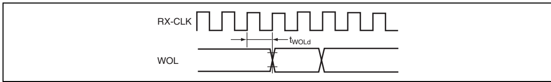
Figure 25.57 WOL Output Timing
