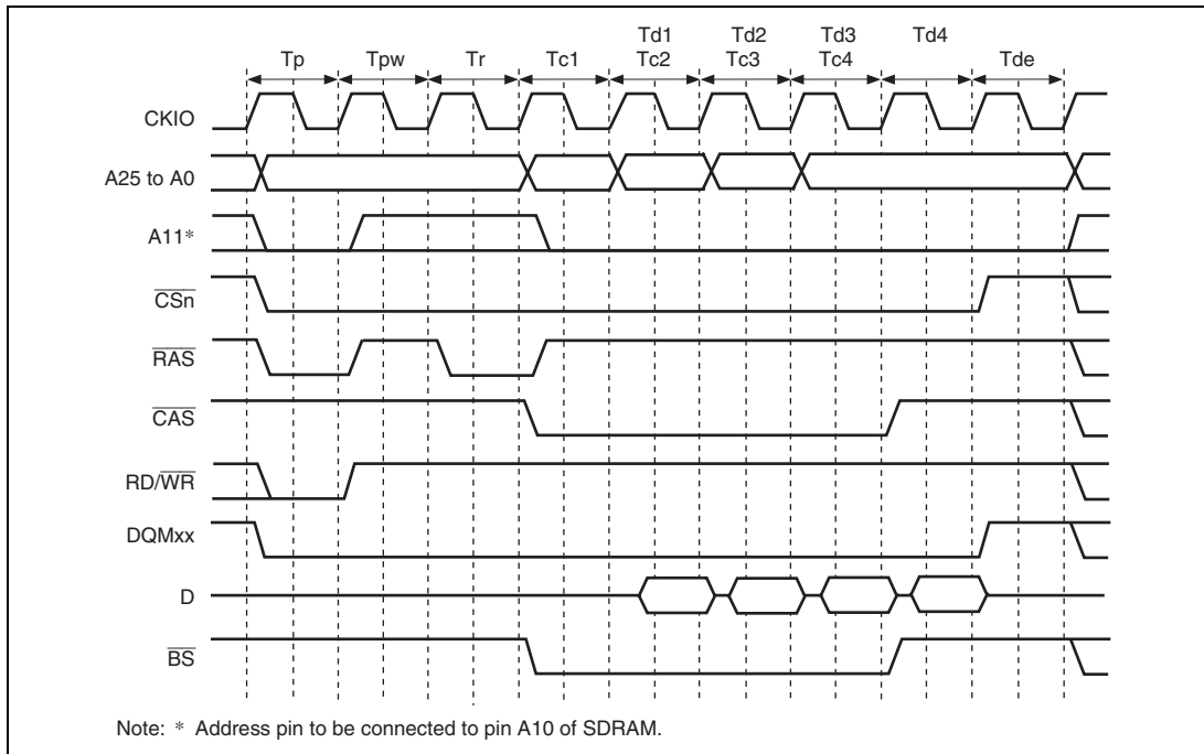
Figure 7.21 Burst Read Timing (Bank Active, Different Row Addresses)
