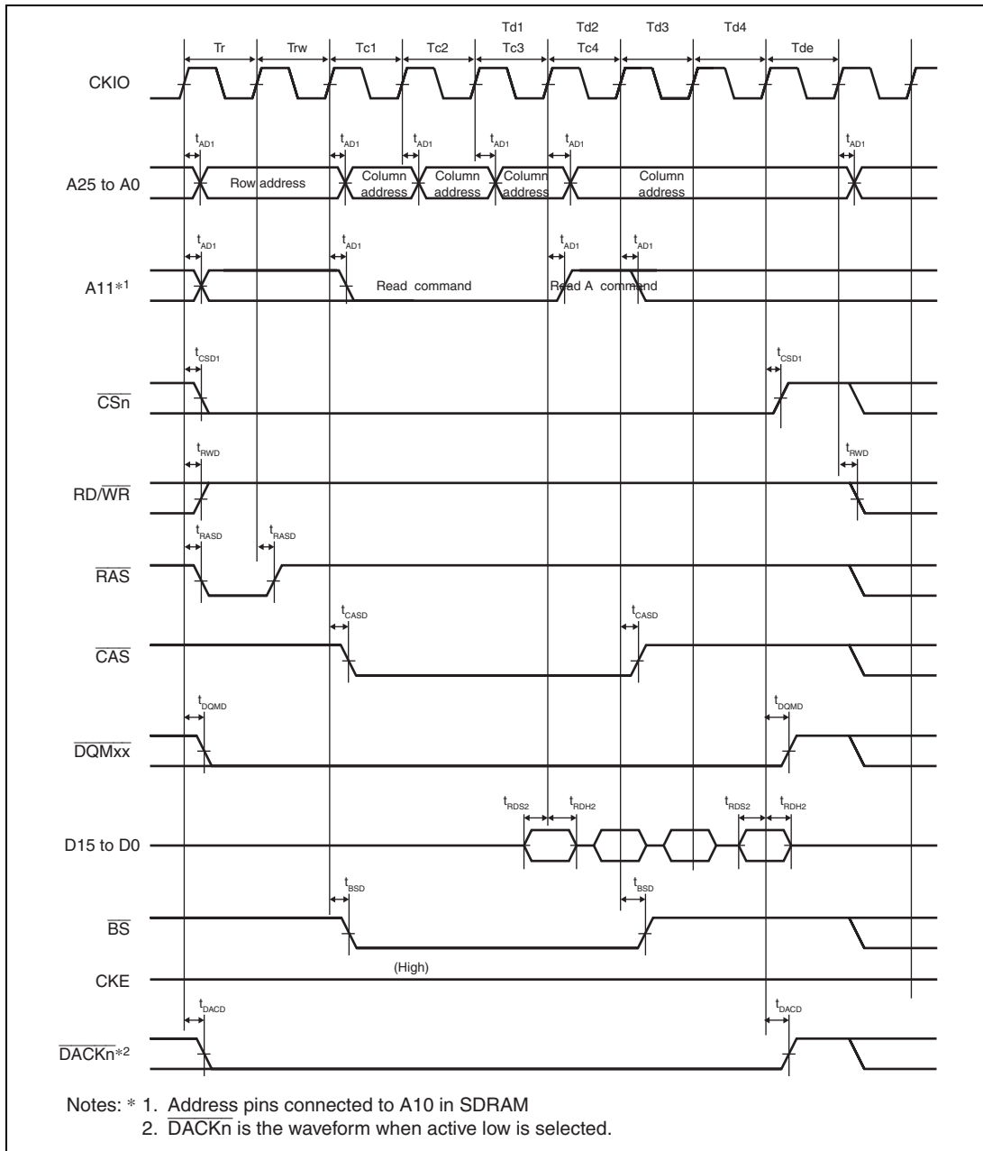
Figure 25.19 Synchronous DRAM Burst Read Bus Cycle (Single Read x 4) (Auto-Precharge, CAS Latency = 2, WTRCD = 1 Cycle, WTRP = 0 Cycle)
