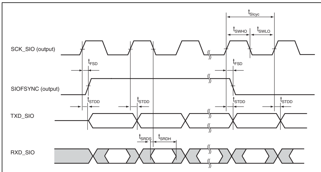
Figure 25.44 SIOF Transmit/Receive Timing (Master Mode 2/Falling Edge Sampling)
