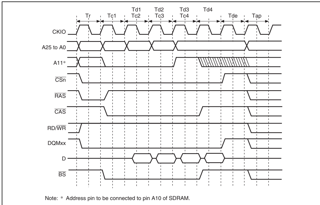
Figure 7.14 Burst Read Basic Timing (Auto Precharge)
