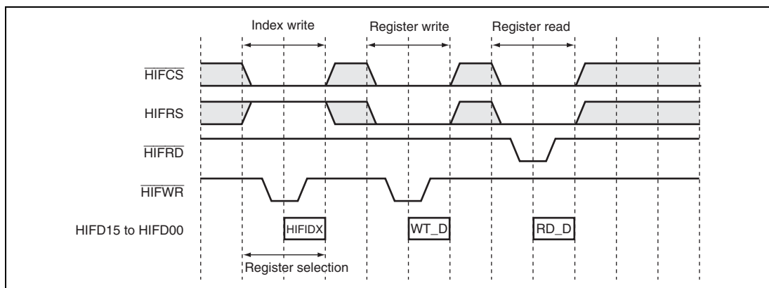
Figure 17.5 HIF Register Settings
