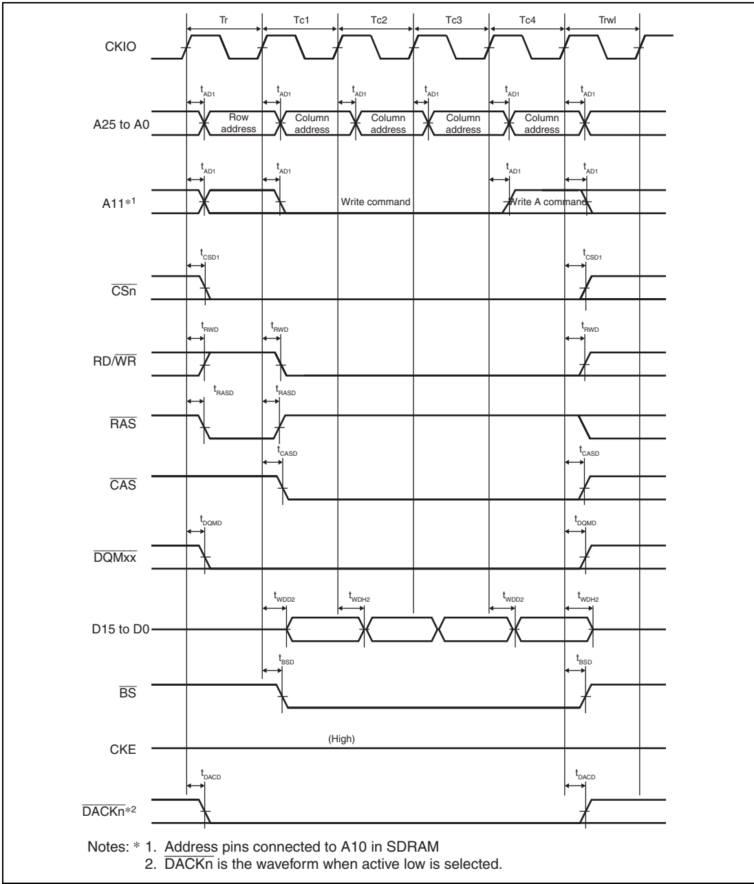
Figure 25.22 Synchronous DRAM Burst Write Bus Cycle (Single Write × 4) (Auto-Precharge, WTRCD = 0 Cycle, TRWL = 1 Cycle)
