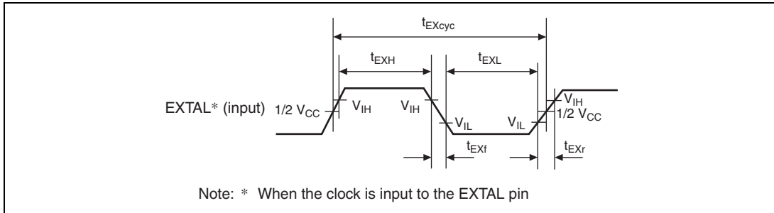
Figure 25.1 External Clock Input Timing
