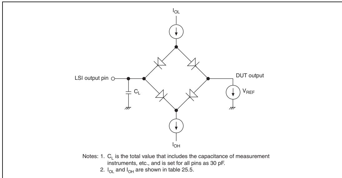
Figure 25.62 Output Load Circuit
