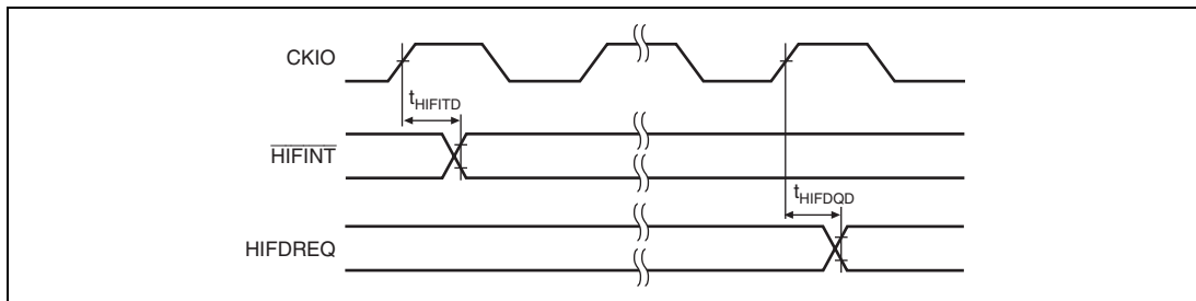
Figure 25.49 \overline{HIFINT} and HIFDREQ Timing
