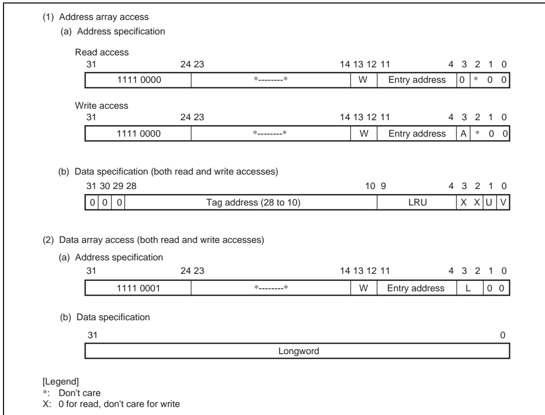
Figure 3.4 Specifying Address and Data for Memory-Mapped Cache Access
