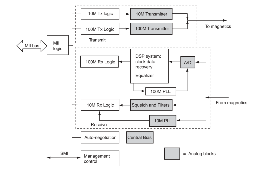
Figure 22.2 Architectural Overview
