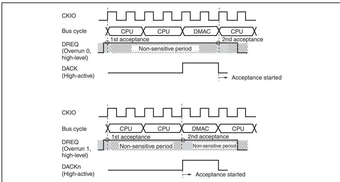
Figure 13.14 Example of DREQ Input Detection in Cycle Steal Mode Level Detection
