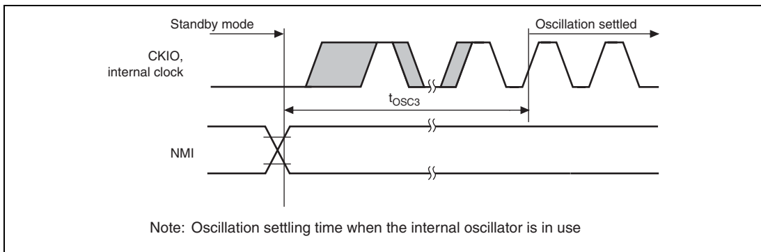
Figure 25.5 Oscillation Settling Timing after Standby Mode (By NMI or IRQ)
