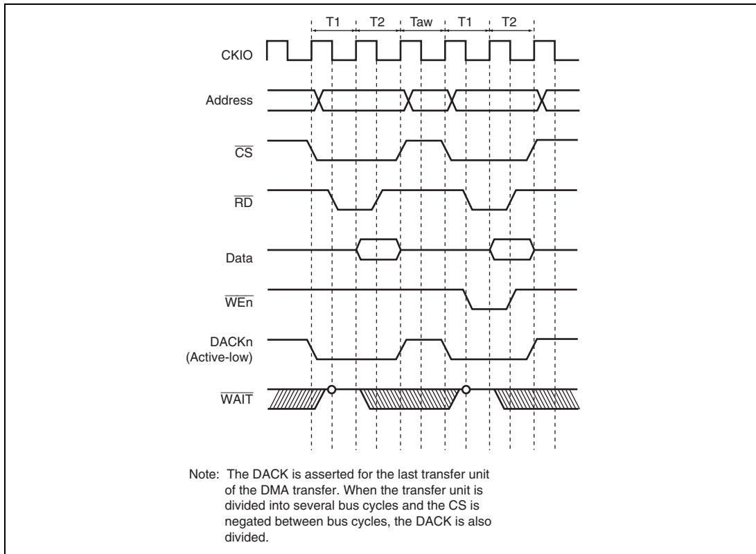
Figure 13.18 Example of BSC Ordinary Memory Access (No Wait, Idle Cycle 1, Longword Access to 16-Bit Device)
