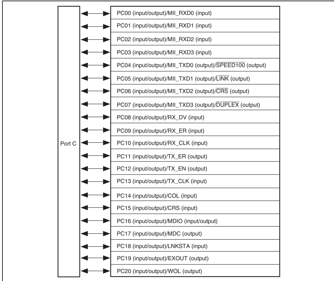
Figure 19.3 Port C
