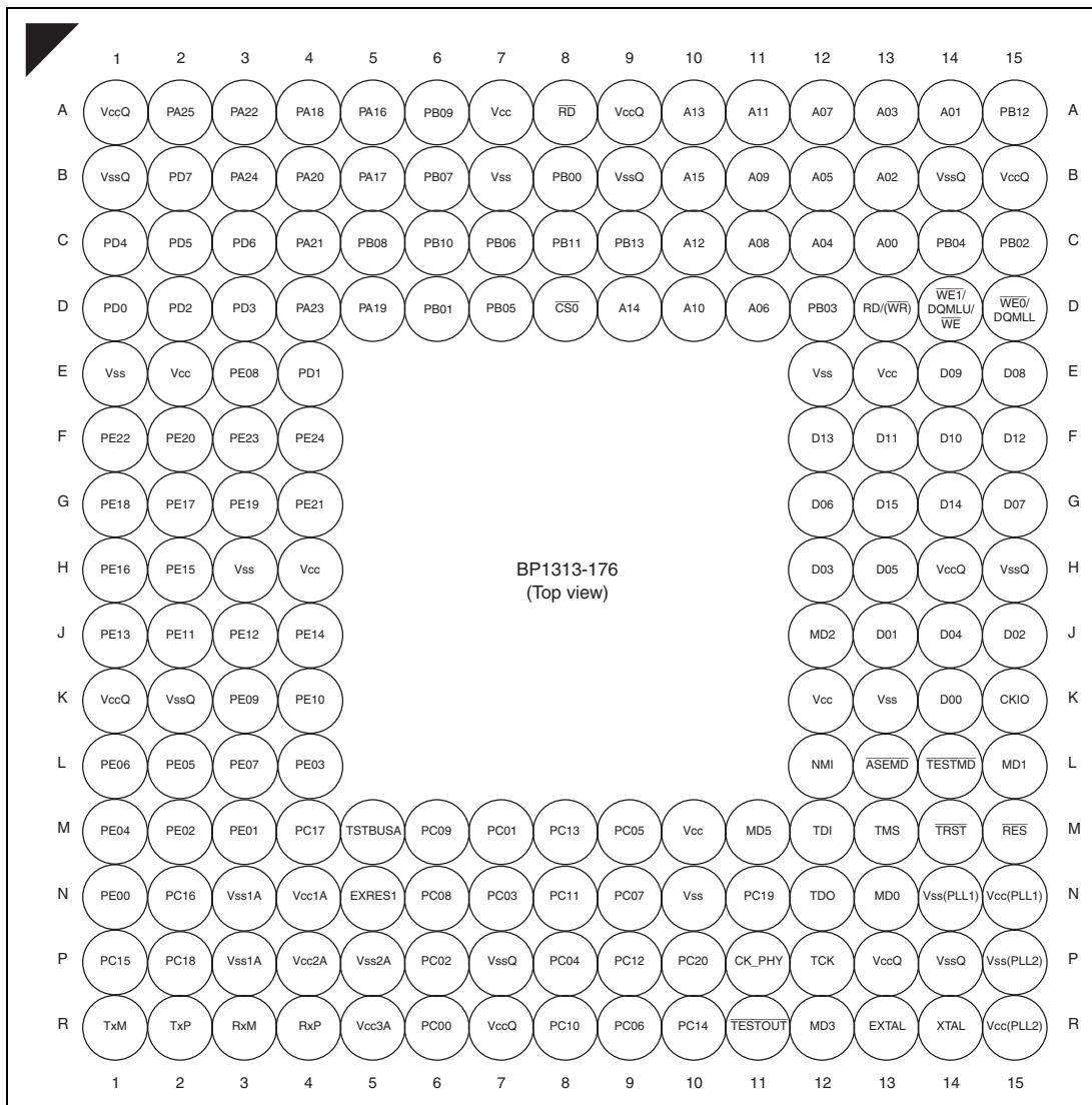
Figure 1.2 Pin Assignments
