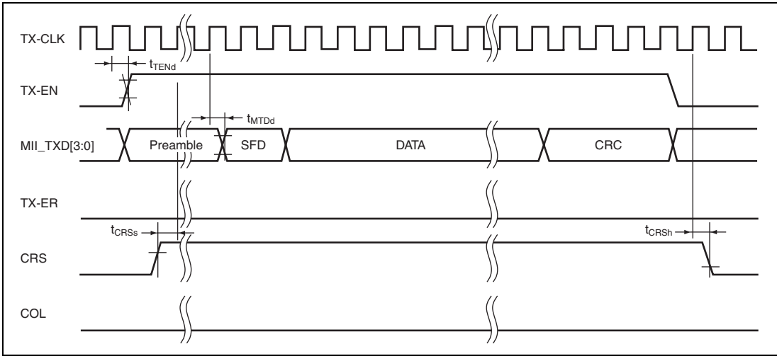
Figure 25.51 MII Transmission Timing (Normal Operation)
