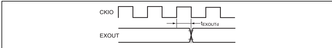
Figure 25.58 EXOUT Output Timing
