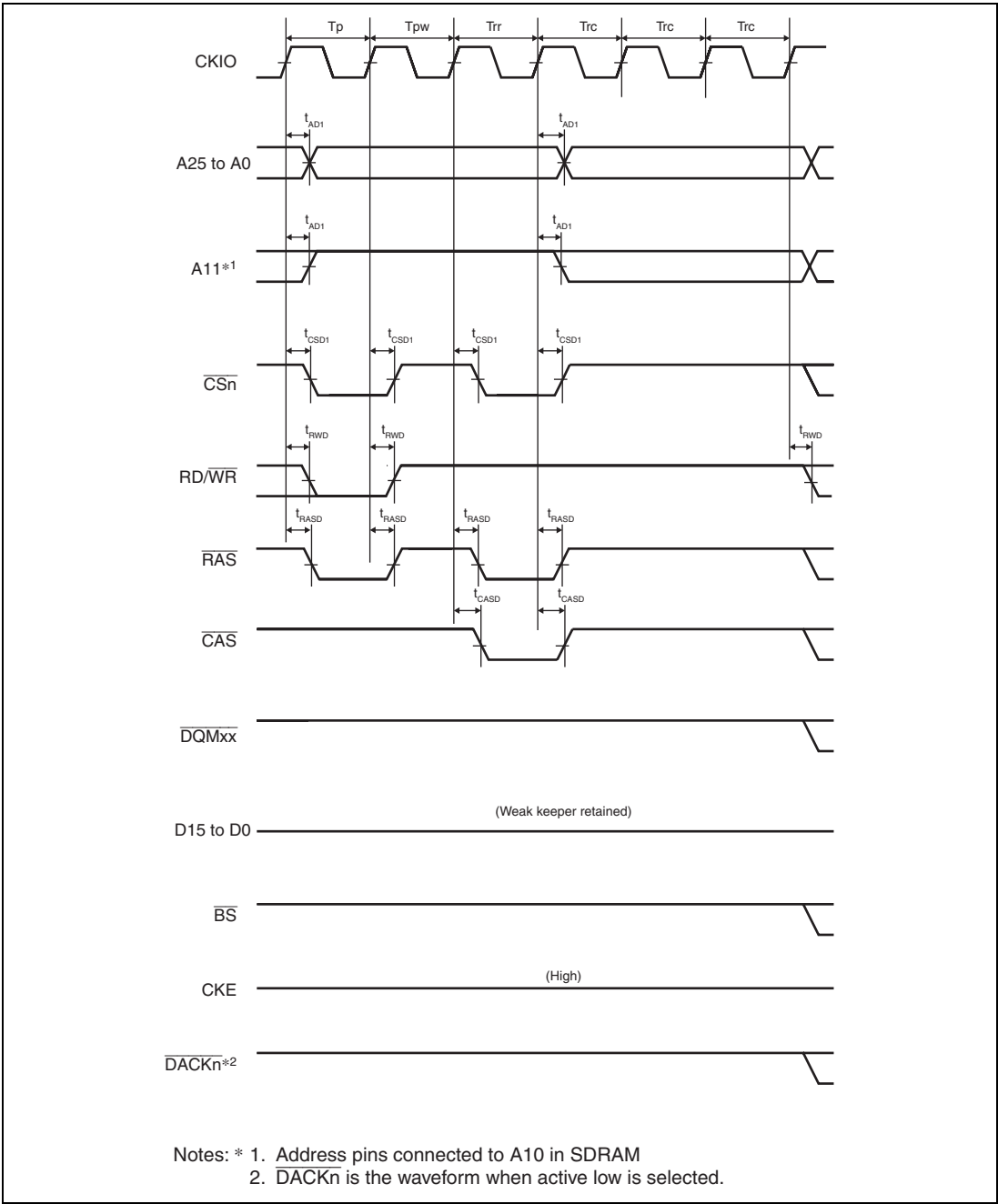
Figure 25.30 Synchronous DRAM Auto-Refreshing Timing (WTRP = 1 Cycle, WTRC = 3 Cycles)
