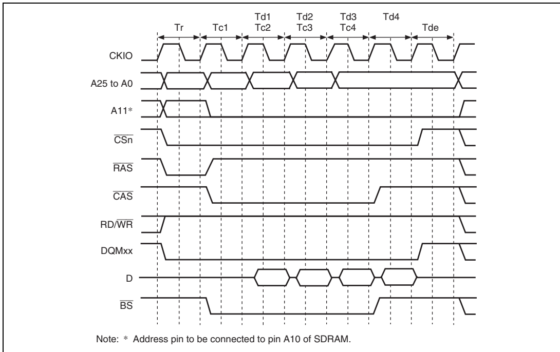
Figure 7.19 Burst Read Timing (No Auto Precharge)
