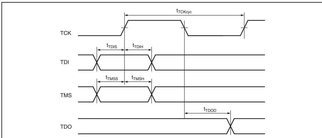
Figure 25.61 H-UDI Data Transmission Timing
