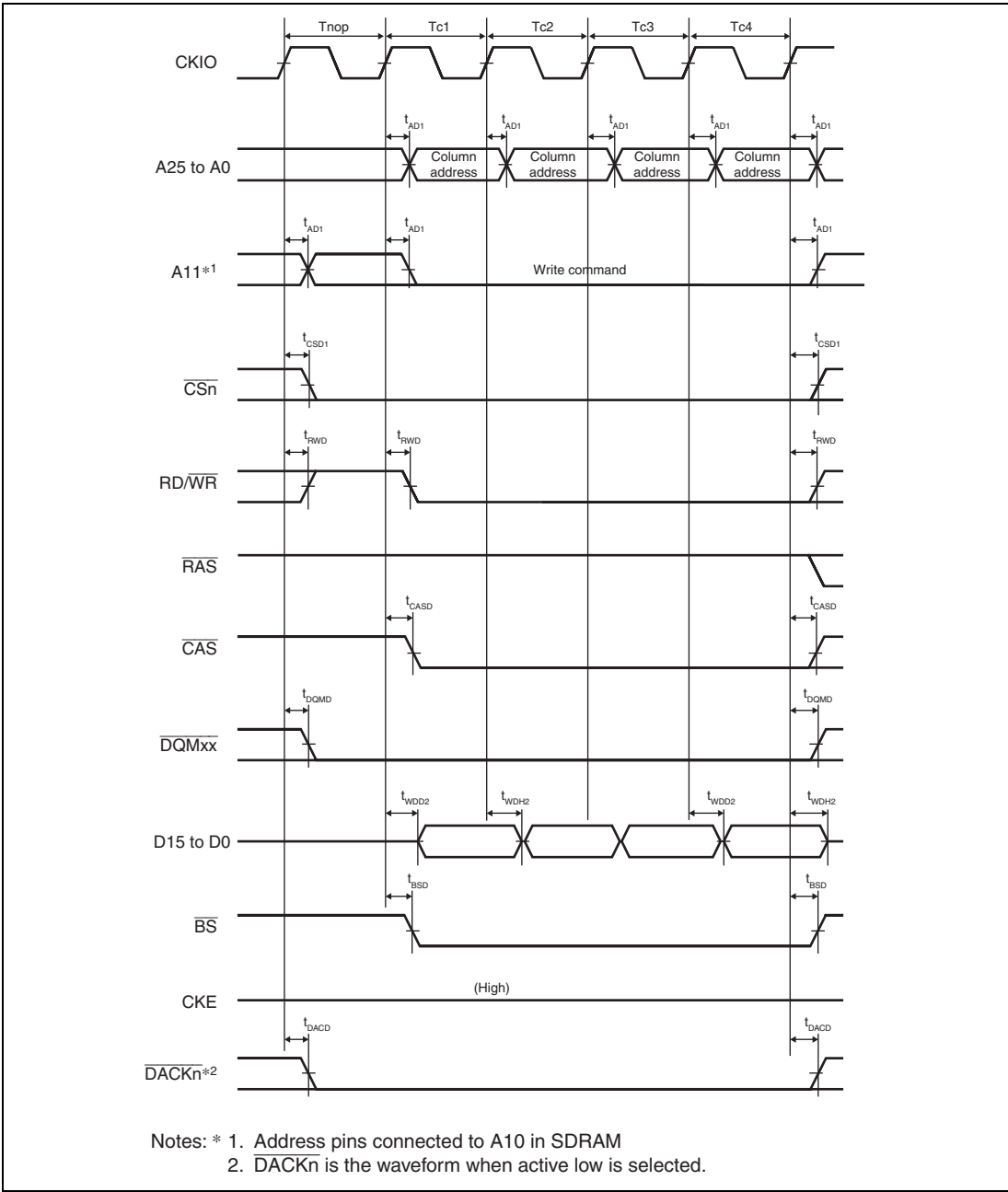
Figure 25.28 Synchronous DRAM Burst Write Bus Cycle (Single Write × 4) (Bank Active Mode: WRITE Command, Same Row Address, WTRCD = 0 Cycle, TRWL = 0 Cycle)
