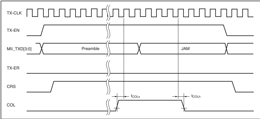
Figure 25.52 MII Transmission Timing (Collision Occurred)
