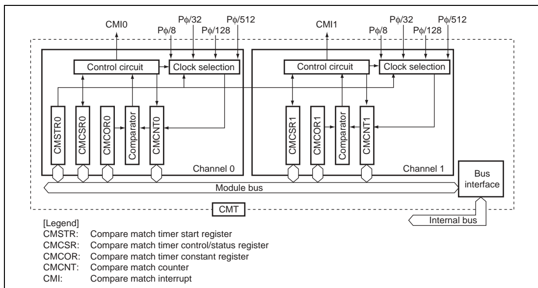
Figure 14.1 Block Diagram of Compare Match Timer
