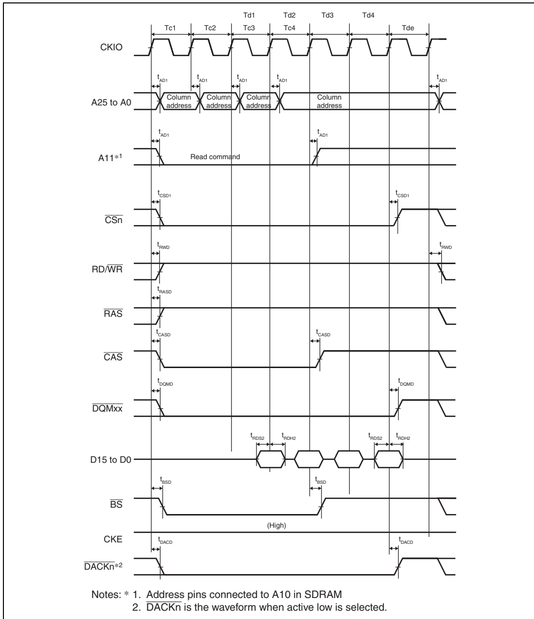
Figure 25.25 Synchronous DRAM Burst Read Bus Cycle (Single Read x 4) (Bank Active Mode: READ Command, Same Row Address, CAS Latency = 2, WTRCD = 0 Cycle)
