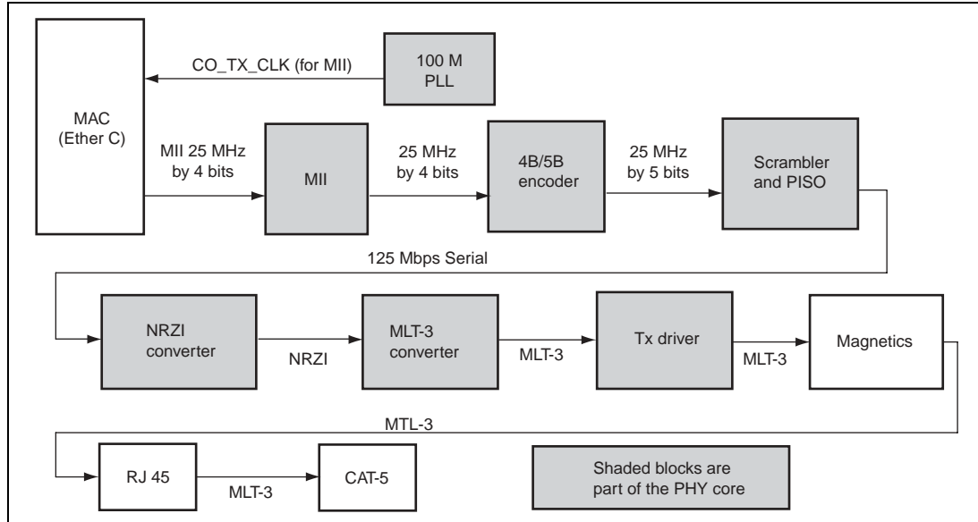
Figure 22.6 100Base-TX Data Path
