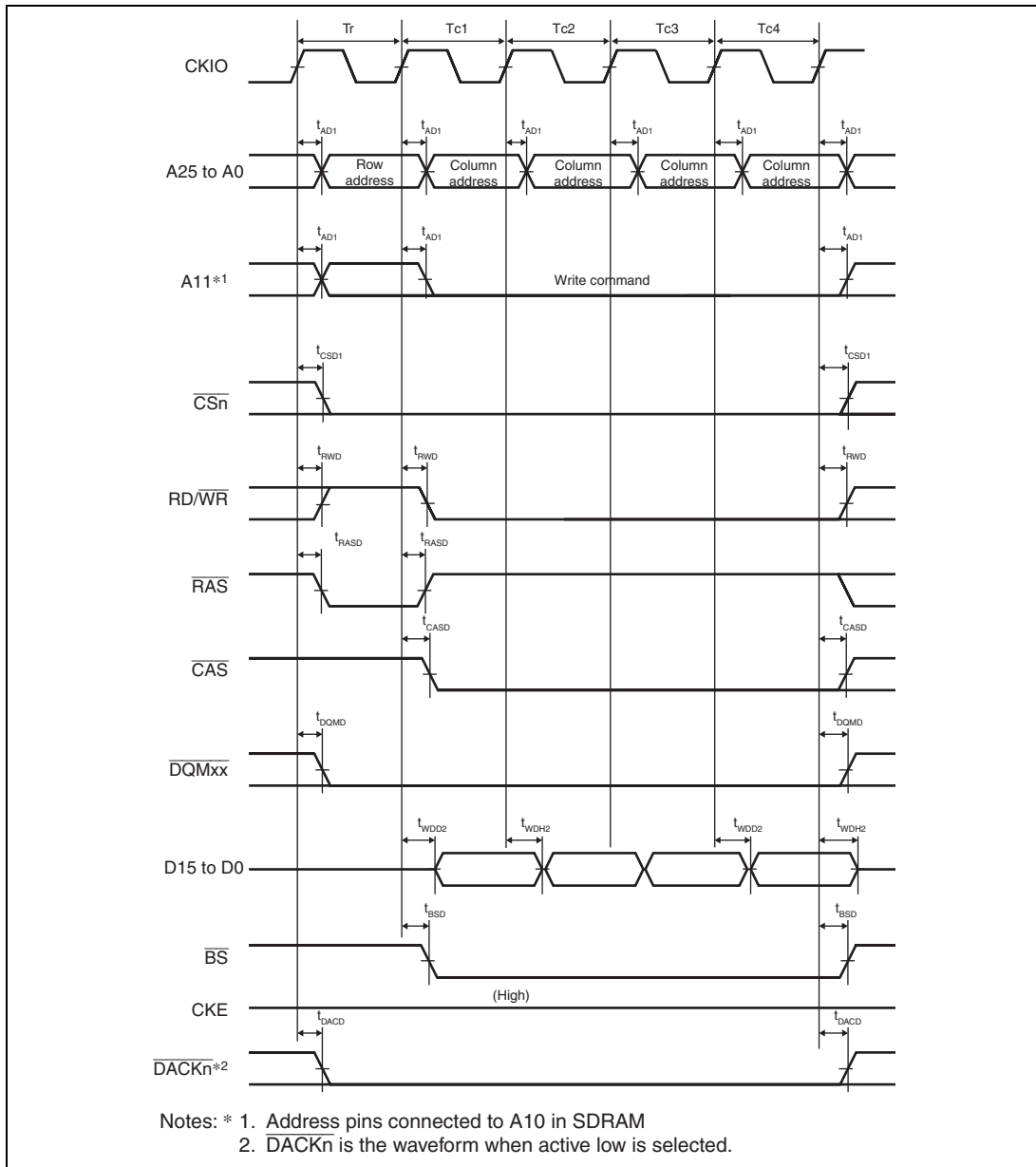
Figure 25.27 Synchronous DRAM Burst Write Bus Cycle (Single Write × 4) (Bank Active Mode: ACT + WRITE Commands, WTRCD = 0 Cycle, TRWL = 0 Cycle)
