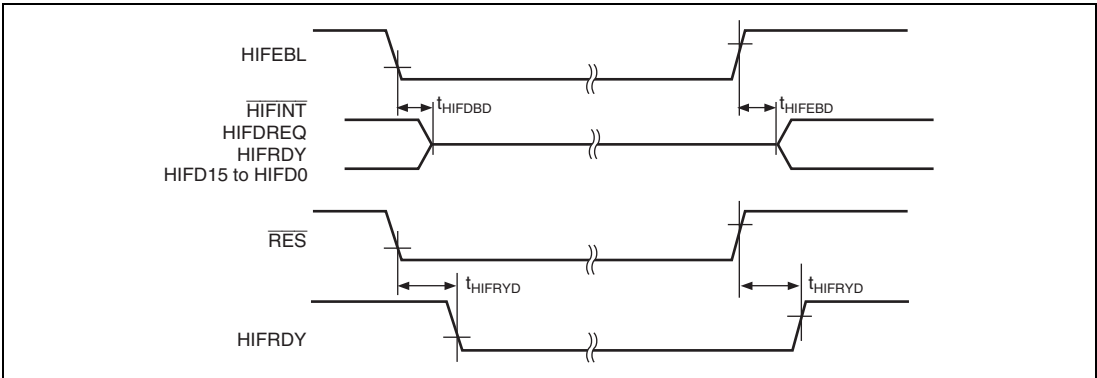
Figure 25.50 HIFRDY and HIF Pin Enable/Disable Timing
