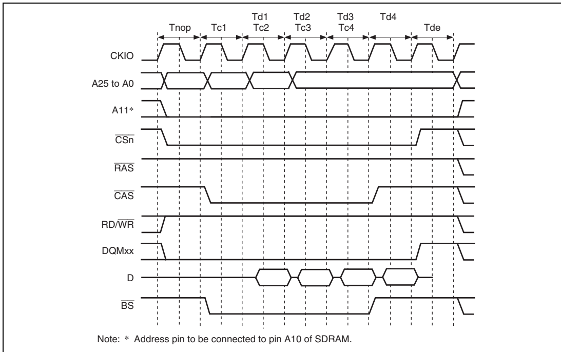
Figure 7.20 Burst Read Timing (Bank Active, Same Row Address)
