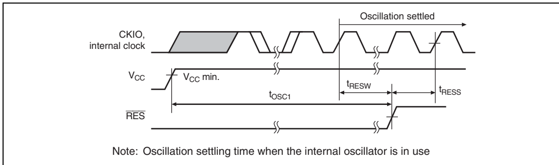
Figure 25.3 Oscillation Settling Timing after Power-On
