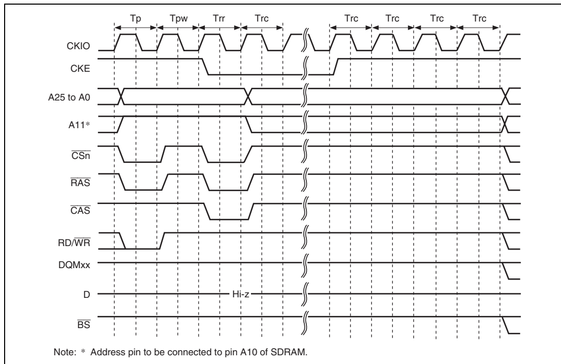
Figure 7.26 Self-Refreshing Timing
