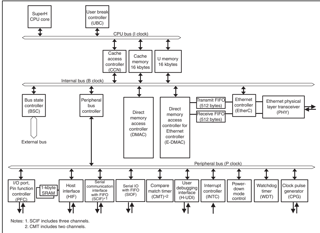
Figure 1.1 Block Diagram
