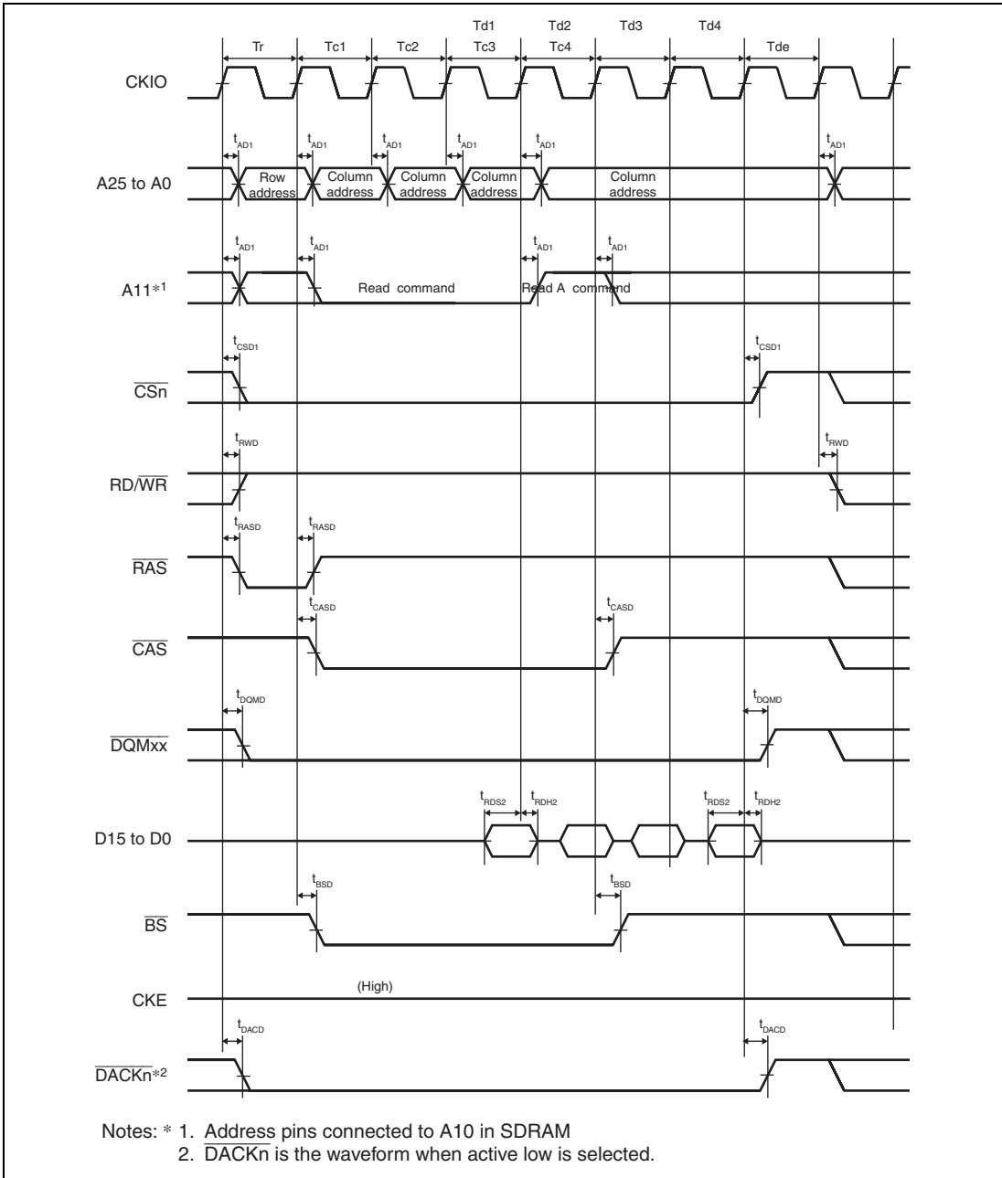
Figure 25.18 Synchronous DRAM Burst Read Bus Cycle (Single Read x 4) (Auto-Precharge, CAS Latency = 2, WTRCD = 0 Cycle, WTRP = 1 Cycle)
