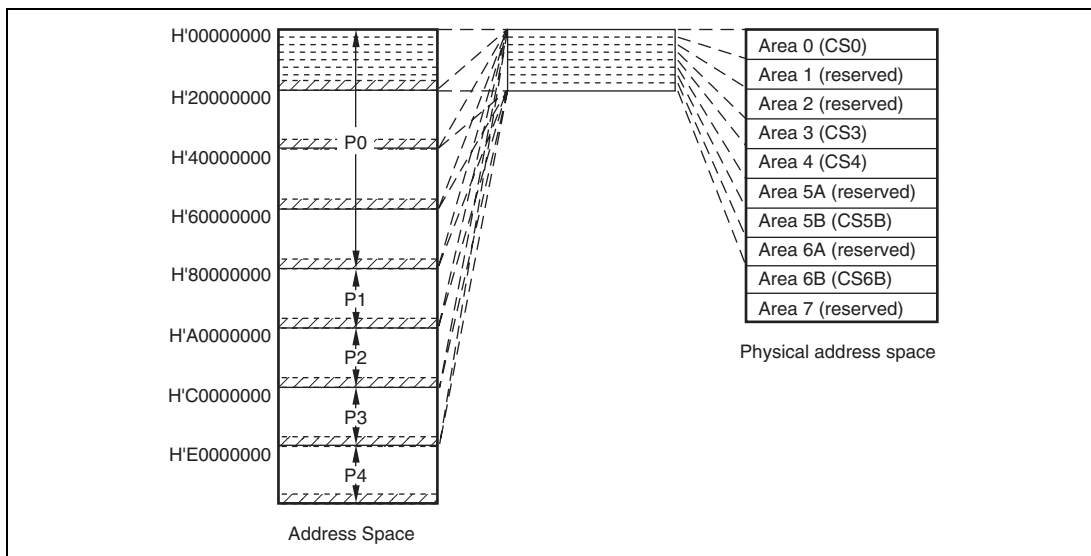
Figure 7.2 Address Space
