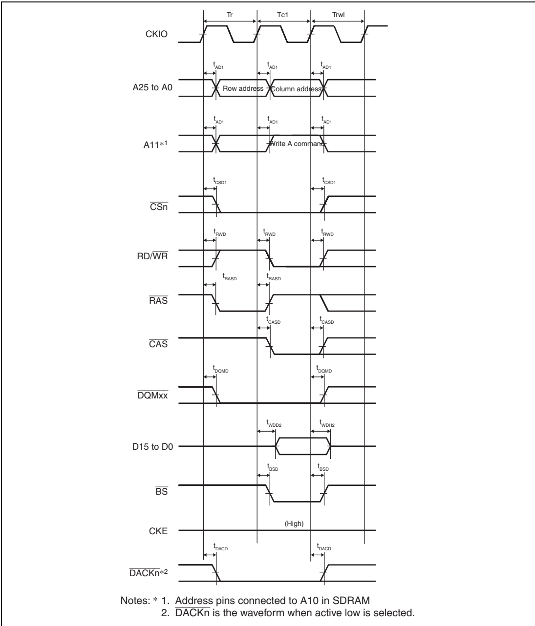
Figure 25.20 Synchronous DRAM Single Write Bus Cycle (Auto-Precharge, TRWL = 1 Cycle)
