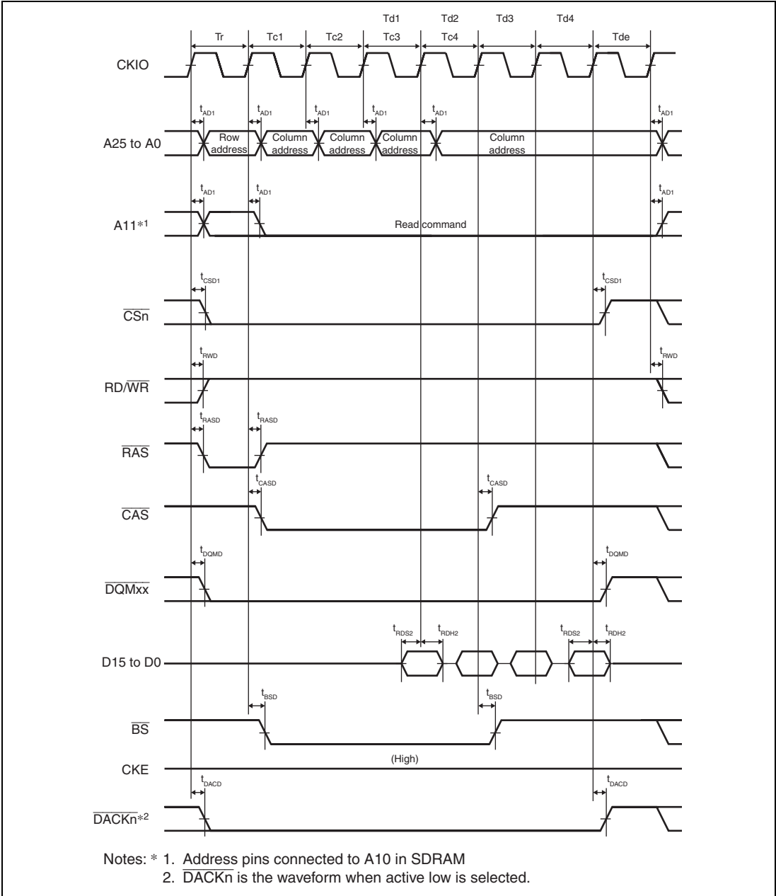
Figure 25.24 Synchronous DRAM Burst Read Bus Cycle (Single Read x 4) (Bank Active Mode: ACT + READ Commands, CAS Latency = 2, WTRCD = 0 Cycle)
