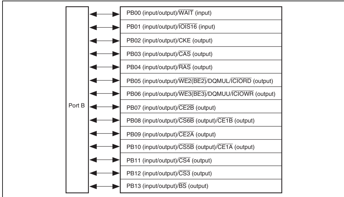
Figure 19.2 Port B
