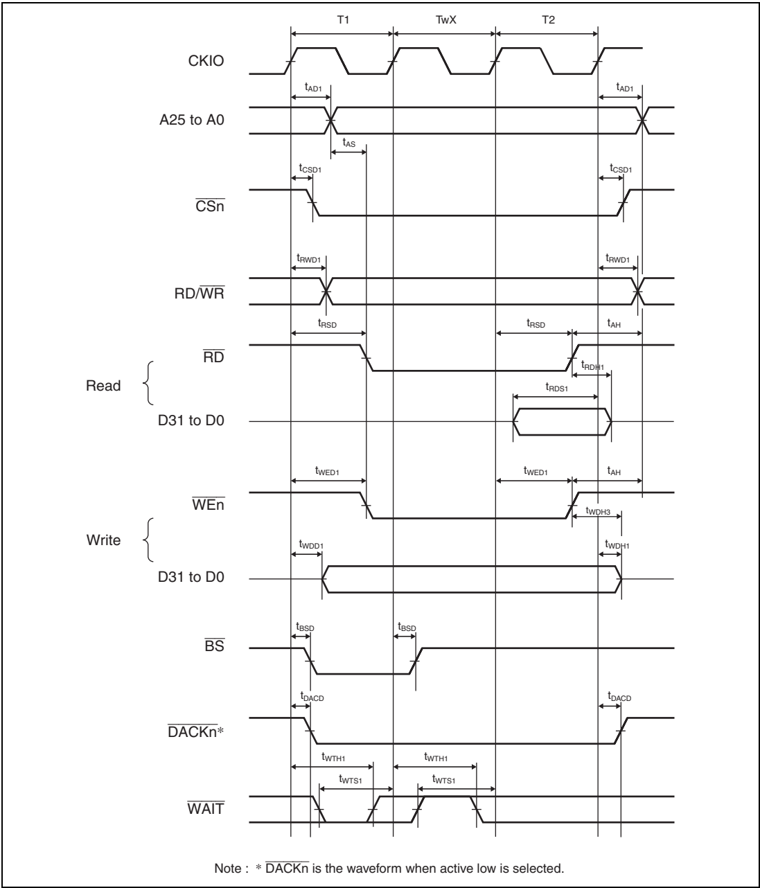
Figure 25.12 Basic Bus Timing: One External Wait Cycle
