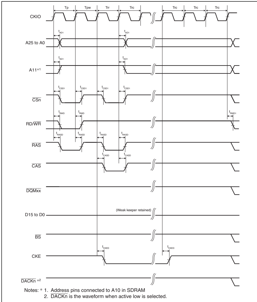
Figure 25.31 Synchronous DRAM Self-Refreshing Timing (WTRP = 1 Cycle)
