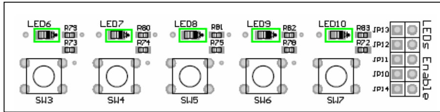
Figure 5-14 User LEDs.
