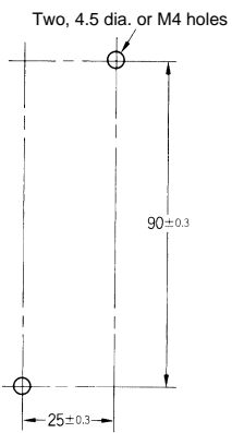
Mounting Holes
