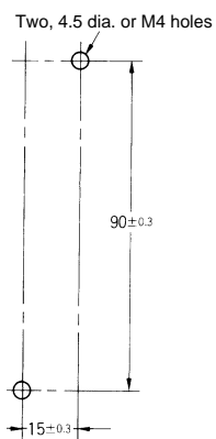
Mounting Holes
