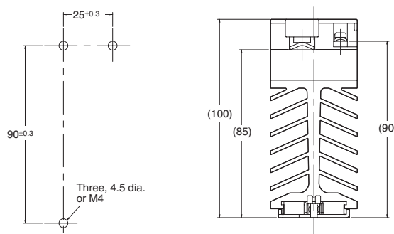
Mounting Holes
