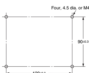
Mounting Holes
