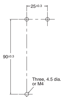
Mounting Holes
