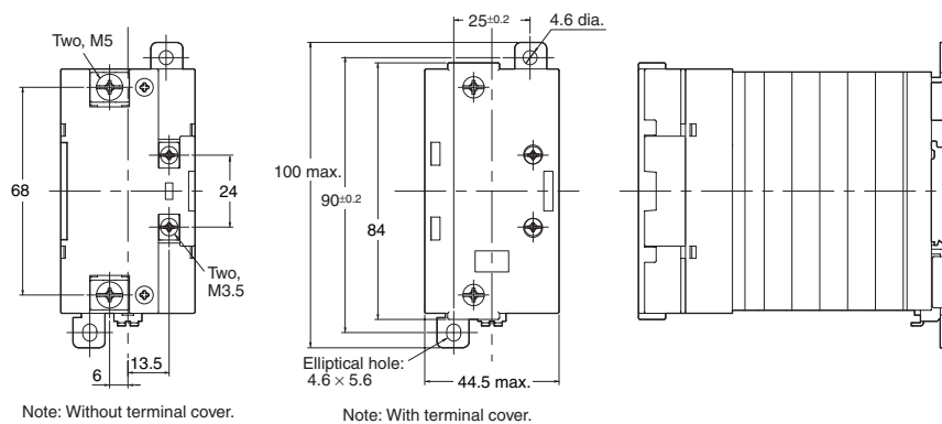
Mounting Holes
