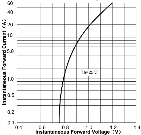
FIG3: Forward Voltage
