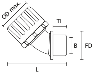
HelGuard fitting, 45° with fixed external thread
