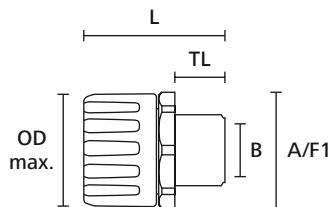
HeliaGuard fitting, straight with fixed external thread
