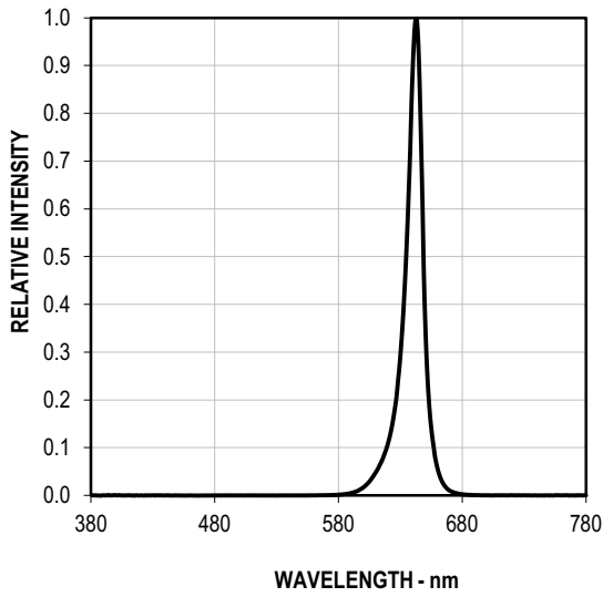
Figure 2: Intensity vs. Wavelength
