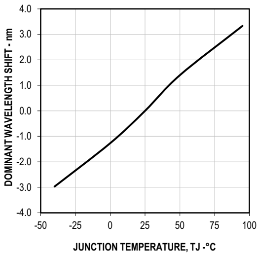
Figure 8: Wavelength vs. Temperature
